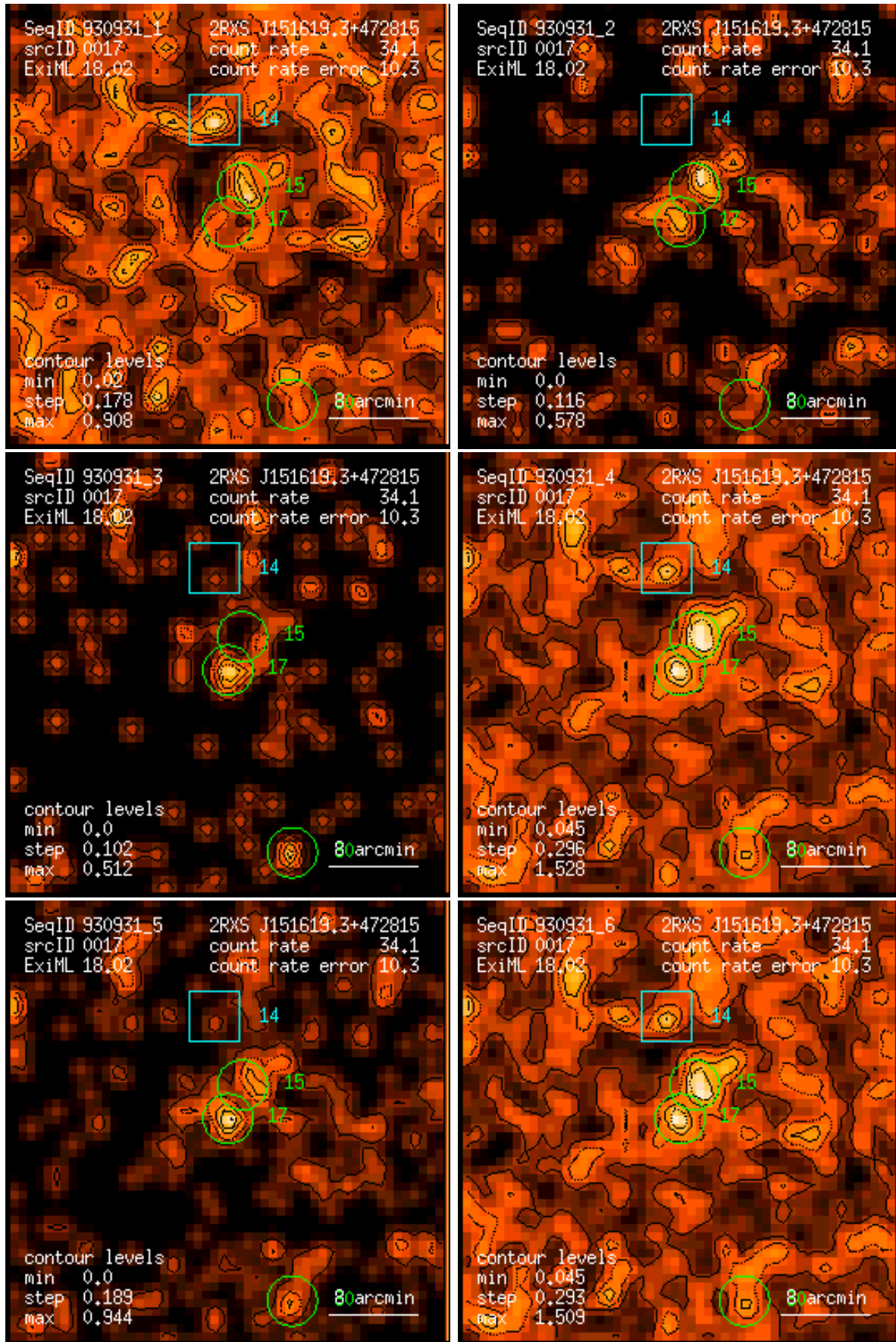
Figure 17: RASS 930931: detection 0017: band rate images, Gaussian filter: (1) PSPC channels 11 – 41, (2) 52 – 90, (3) 91 – 201, (4) 11 – 235, (5) 52 – 201, (6) 11 – 201. Broad band rates in counts/ks. Band rate contour levels in counts/ks/arcmin 2 .
