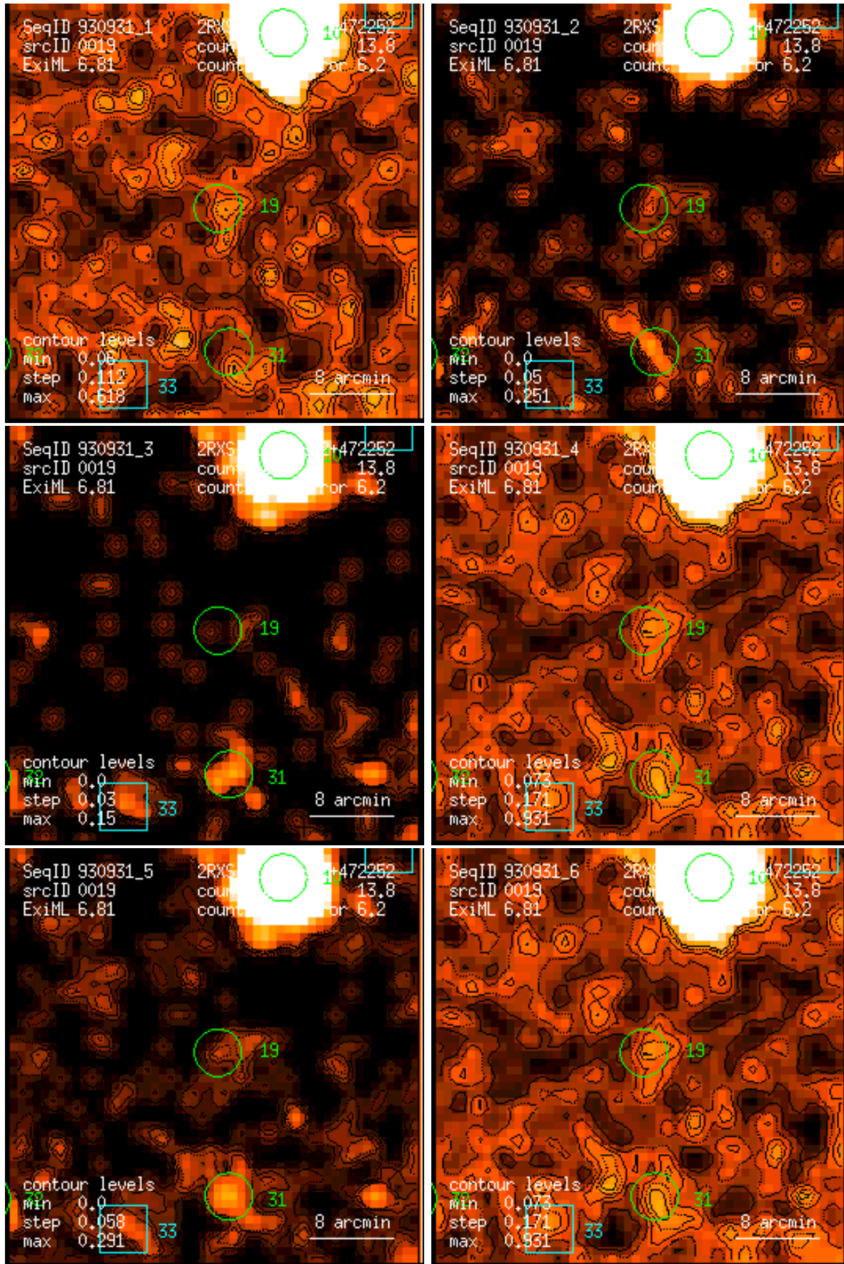
Figure 19: RASS 930931: detection 0019: band rate images, Gaussian filter: (1) PSPC channels 11 – 41, (2) 52 – 90, (3) 91 – 201, (4) 11 – 235, (5) 52 – 201, (6) 11 – 201. Broad band rates in counts/ks. Band rate contour levels in counts/ks/arcmin 2 .
