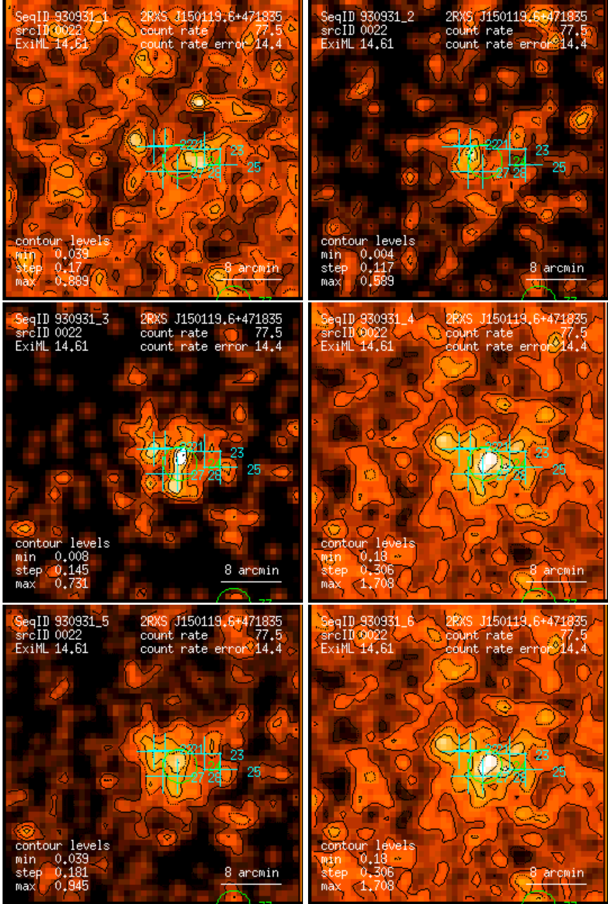
Figure 22: RASS 930931: detection 0022: band rate images, Gaussian filter: (1) PSPC channels 11 – 41, (2) 52 – 90, (3) 91 – 201, (4) 11 – 235, (5) 52 – 201, (6) 11 – 201. Broad band rates in counts/ks. Band rate contour levels in counts/ks/arcmin 2 .
