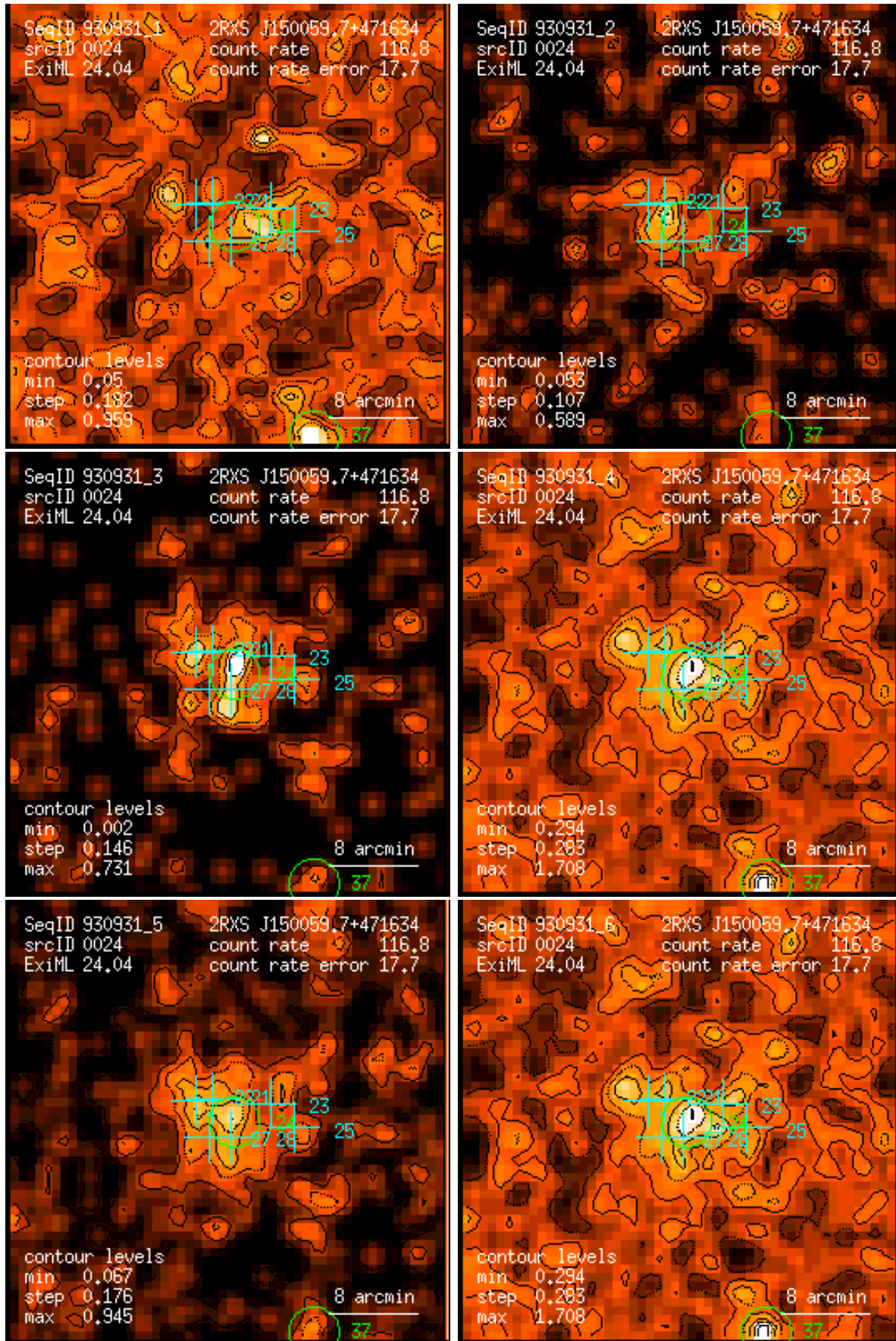
Figure 24: RASS 930931: detection 0024: band rate images, Gaussian filter: (1) PSPC channels 11 – 41, (2) 52 – 90, (3) 91 – 201, (4) 11 – 235, (5) 52 – 201, (6) 11 – 201. Broad band rates in counts/ks. Band rate contour levels in counts/ks/arcmin 2 .
