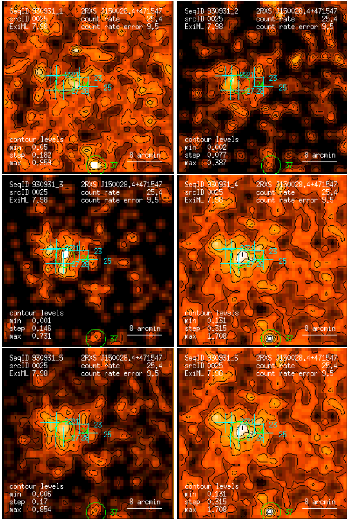
Figure 25: RASS 930931: detection 0025: band rate images, Gaussian filter: (1) PSPC channels 11 – 41, (2) 52 – 90, (3) 91 – 201, (4) 11 – 235, (5) 52 – 201, (6) 11 – 201. Broad band rates in counts/ks. Band rate contour levels in counts/ks/arcmin 2 .
