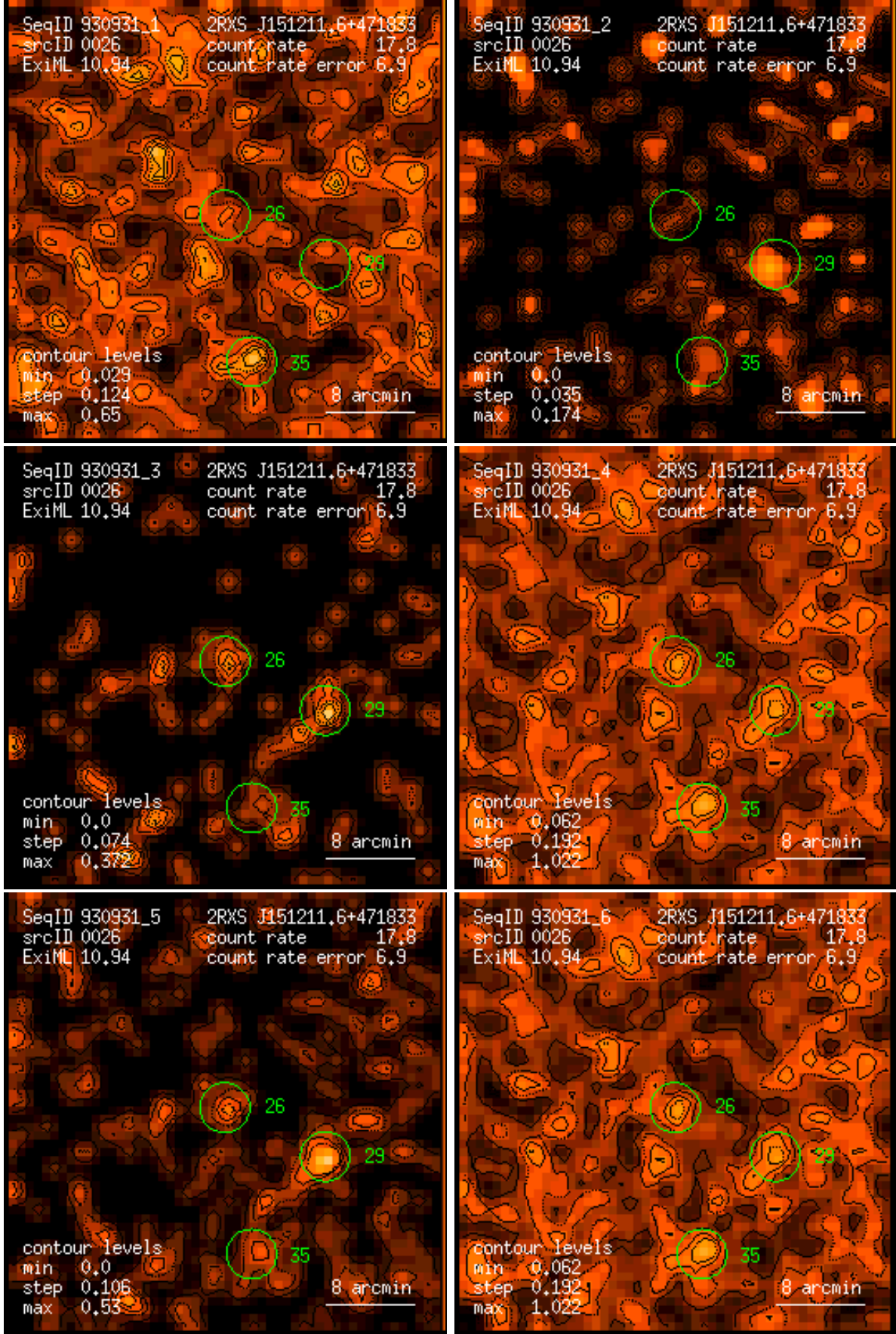
Figure 26: RASS 930931: detection 0026: band rate images, Gaussian filter: (1) PSPC channels 11 – 41, (2) 52 – 90, (3) 91 – 201, (4) 11 – 235, (5) 52 – 201, (6) 11 – 201. Broad band rates in counts/ks. Band rate contour levels in counts/ks/arcmin 2 .
