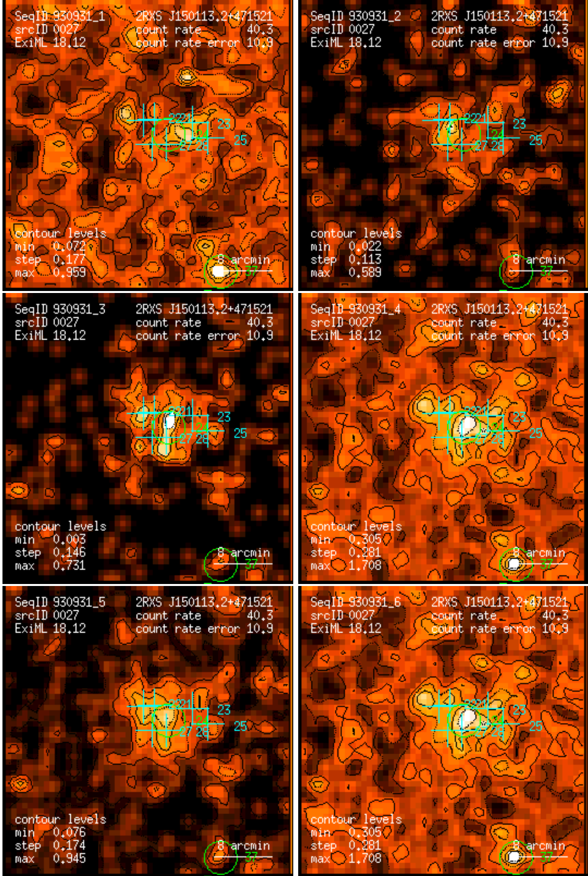
Figure 27: RASS 930931: detection 0027: band rate images, Gaussian filter: (1) PSPC channels 11 – 41, (2) 52 – 90, (3) 91 – 201, (4) 11 – 235, (5) 52 – 201, (6) 11 – 201. Broad band rates in counts/ks. Band rate contour levels in counts/ks/arcmin 2 .
