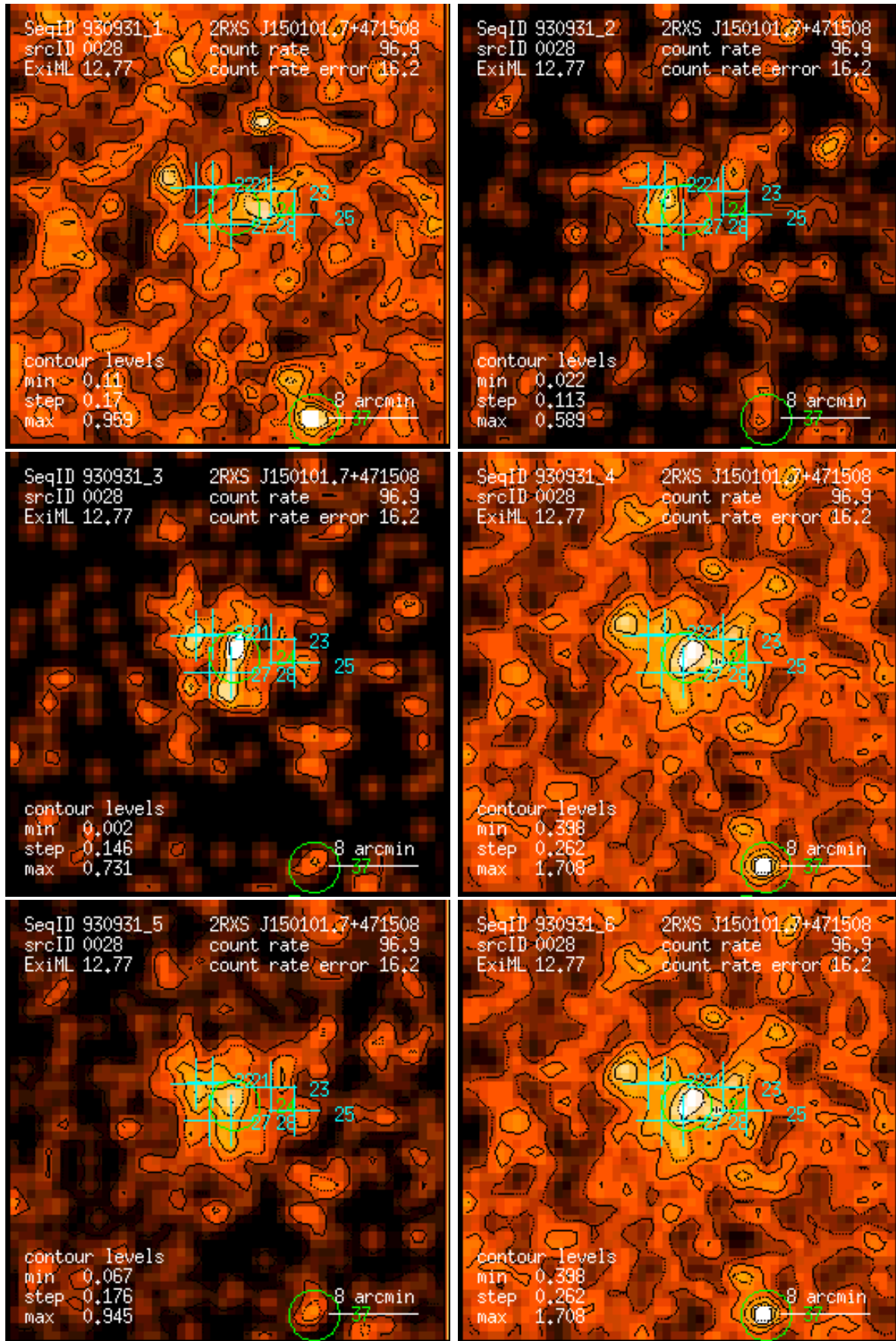
Figure 28: RASS 930931: detection 0028: band rate images, Gaussian filter: (1) PSPC channels 11 – 41, (2) 52 – 90, (3) 91 – 201, (4) 11 – 235, (5) 52 – 201, (6) 11 – 201. Broad band rates in counts/ks. Band rate contour levels in counts/ks/arcmin 2 .
