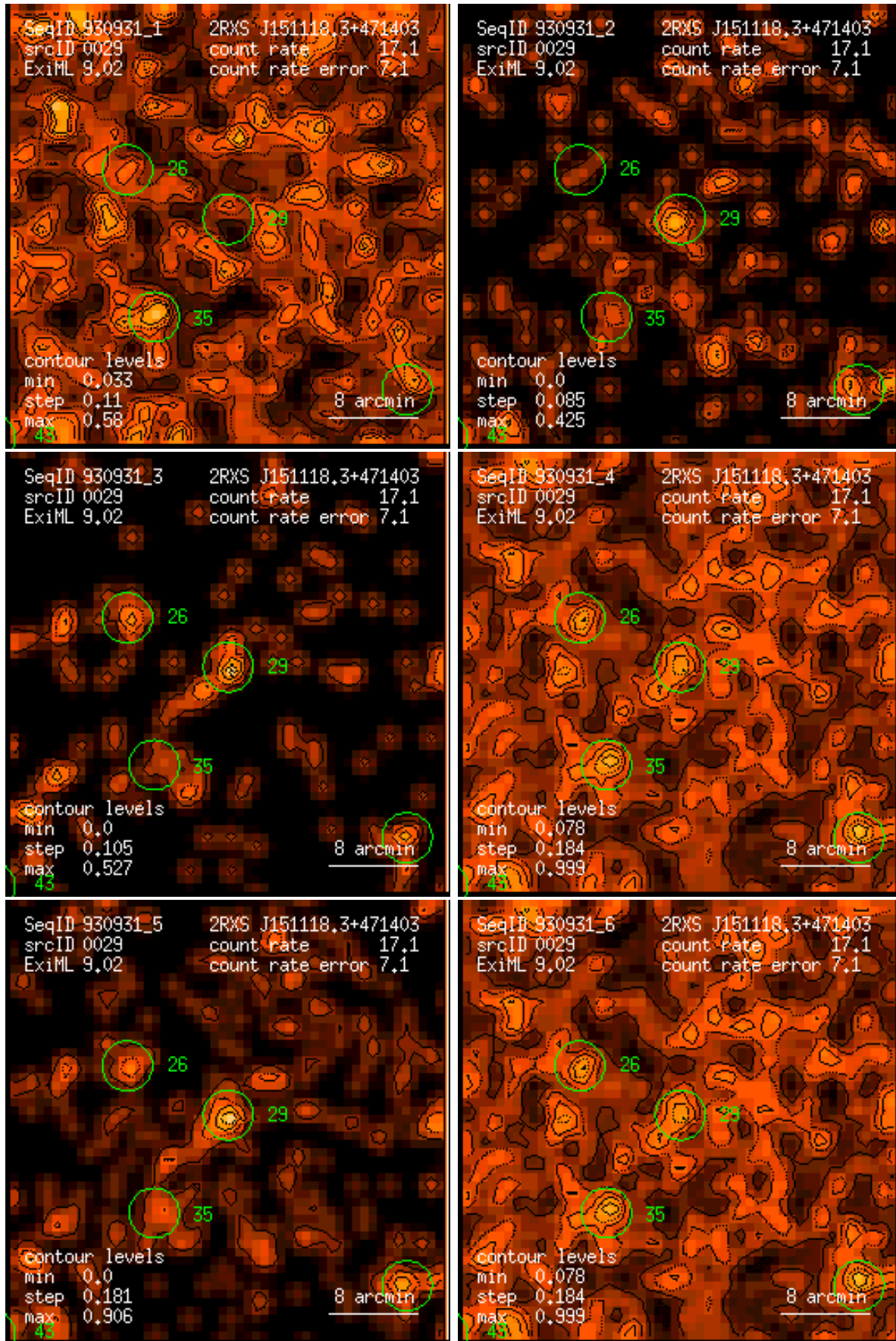
Figure 29: RASS 930931: detection 0029: band rate images, Gaussian filter: (1) PSPC channels 11 – 41, (2) 52 – 90, (3) 91 – 201, (4) 11 – 235, (5) 52 – 201, (6) 11 – 201. Broad band rates in counts/ks. Band rate contour levels in counts/ks/arcmin 2 .
