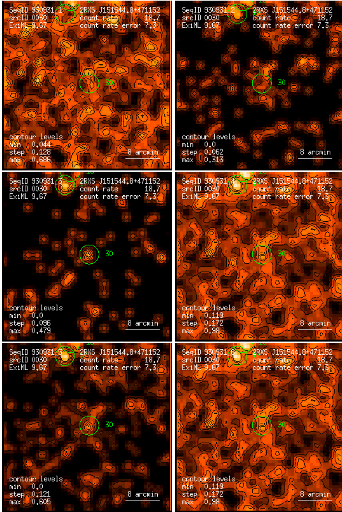
Figure 30: RASS 930931: detection 0030: band rate images, Gaussian filter: (1) PSPC channels 11 – 41, (2) 52 – 90, (3) 91 – 201, (4) 11 – 235, (5) 52 – 201, (6) 11 – 201. Broad band rates in counts/ks. Band rate contour levels in counts/ks/arcmin 2 .
