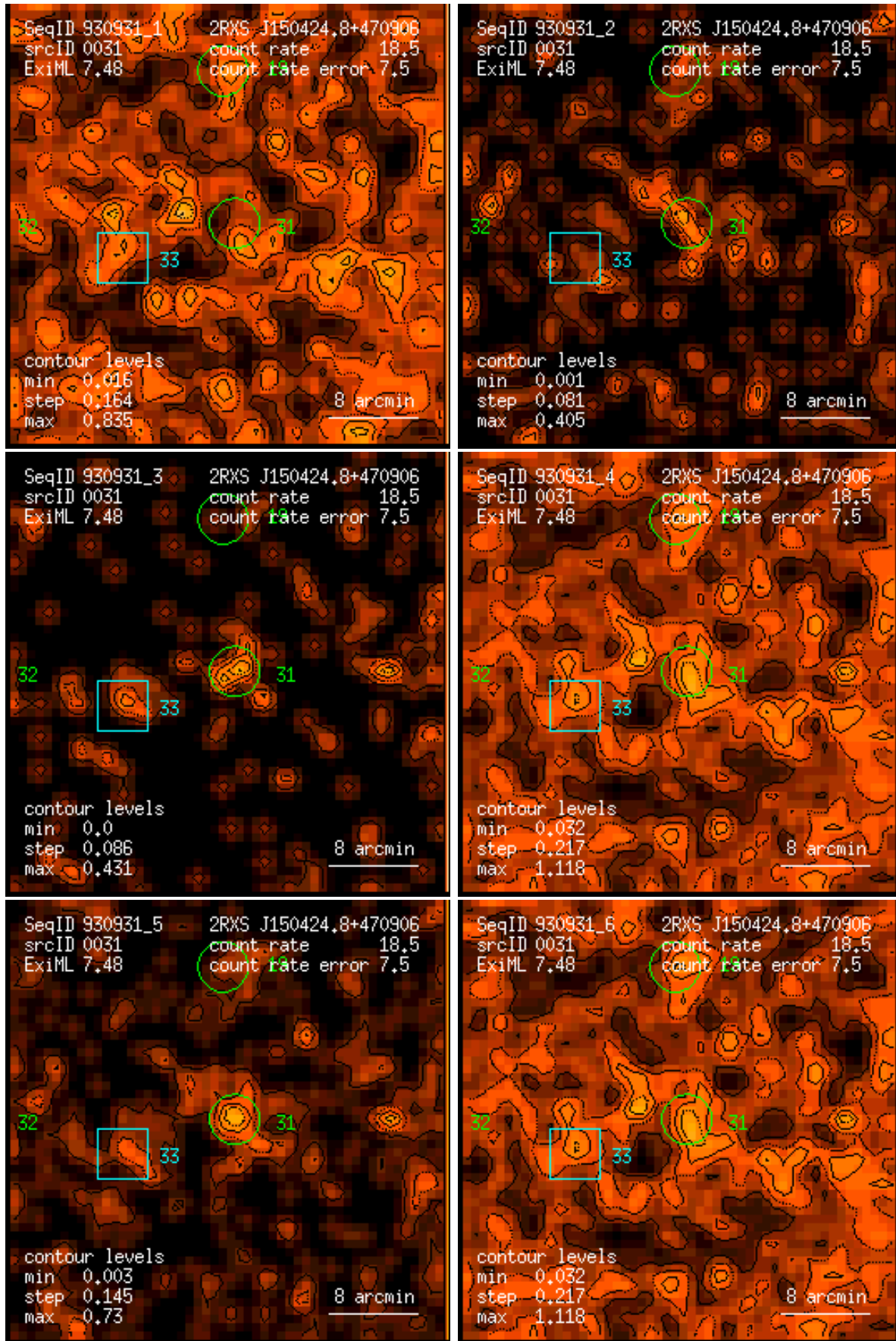
Figure 31: RASS 930931: detection 0031: band rate images, Gaussian filter: (1) PSPC channels 11 – 41, (2) 52 – 90, (3) 91 – 201, (4) 11 – 235, (5) 52 – 201, (6) 11 – 201. Broad band rates in counts/ks. Band rate contour levels in counts/ks/arcmin 2 .
