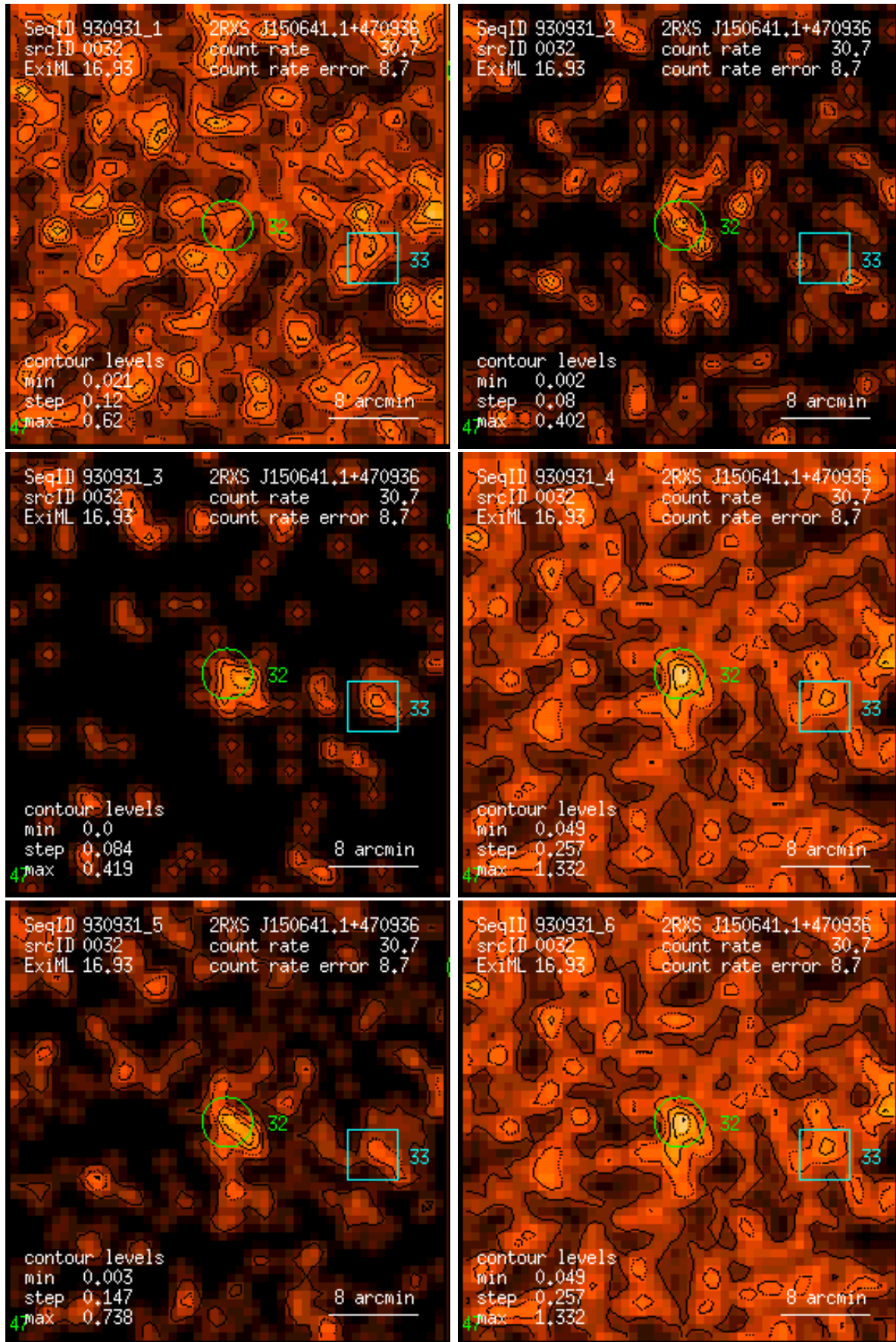
Figure 32: RASS 930931: detection 0032: band rate images, Gaussian filter: (1) PSPC channels 11 – 41, (2) 52 – 90, (3) 91 – 201, (4) 11 – 235, (5) 52 – 201, (6) 11 – 201. Broad band rates in counts/ks. Band rate contour levels in counts/ks/arcmin 2 .
