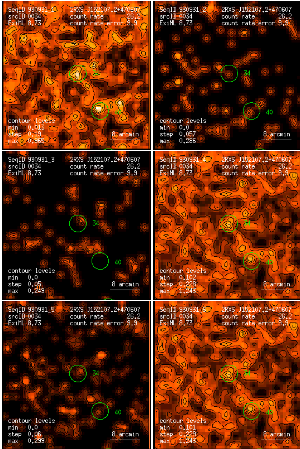
Figure 34: RASS 930931: detection 0034: band rate images, Gaussian filter: (1) PSPC channels 11 – 41, (2) 52 – 90, (3) 91 – 201, (4) 11 – 235, (5) 52 – 201, (6) 11 – 201. Broad band rates in counts/ks. Band rate contour levels in counts/ks/arcmin 2 .
