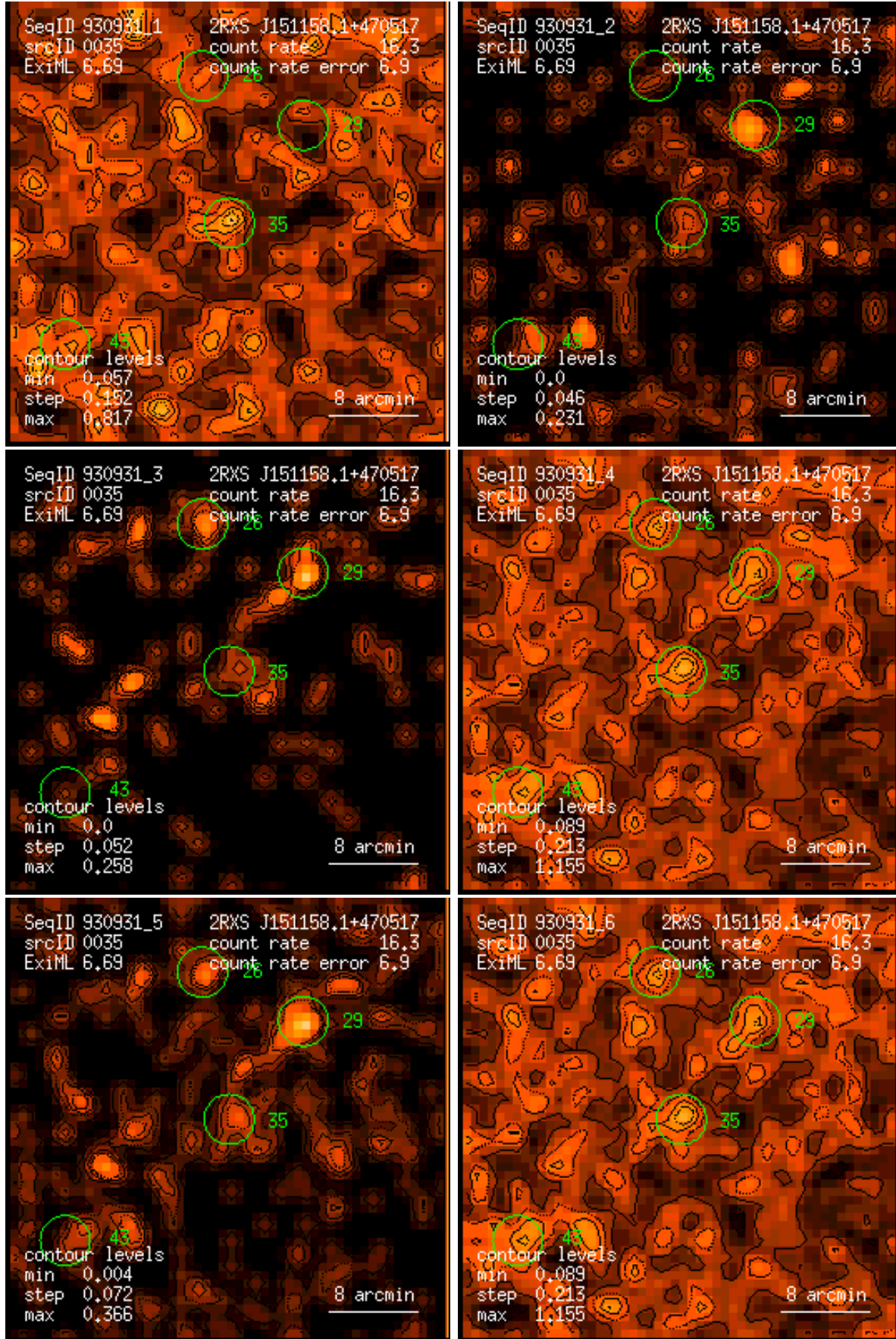
Figure 35: RASS 930931: detection 0035: band rate images, Gaussian filter: (1) PSPC channels 11 – 41, (2) 52 – 90, (3) 91 – 201, (4) 11 – 235, (5) 52 – 201, (6) 11 – 201. Broad band rates in counts/ks. Band rate contour levels in counts/ks/arcmin 2 .
