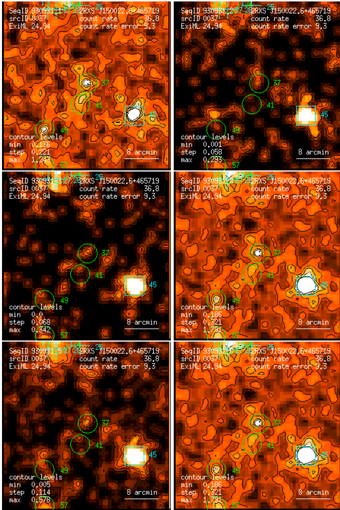
Figure 37: RASS 930931: detection 0037: band rate images, Gaussian filter: (1) PSPC channels 11 – 41, (2) 52 – 90, (3) 91 – 201, (4) 11 – 235, (5) 52 – 201, (6) 11 – 201. Broad band rates in counts/ks. Band rate contour levels in counts/ks/arcmin 2 .
