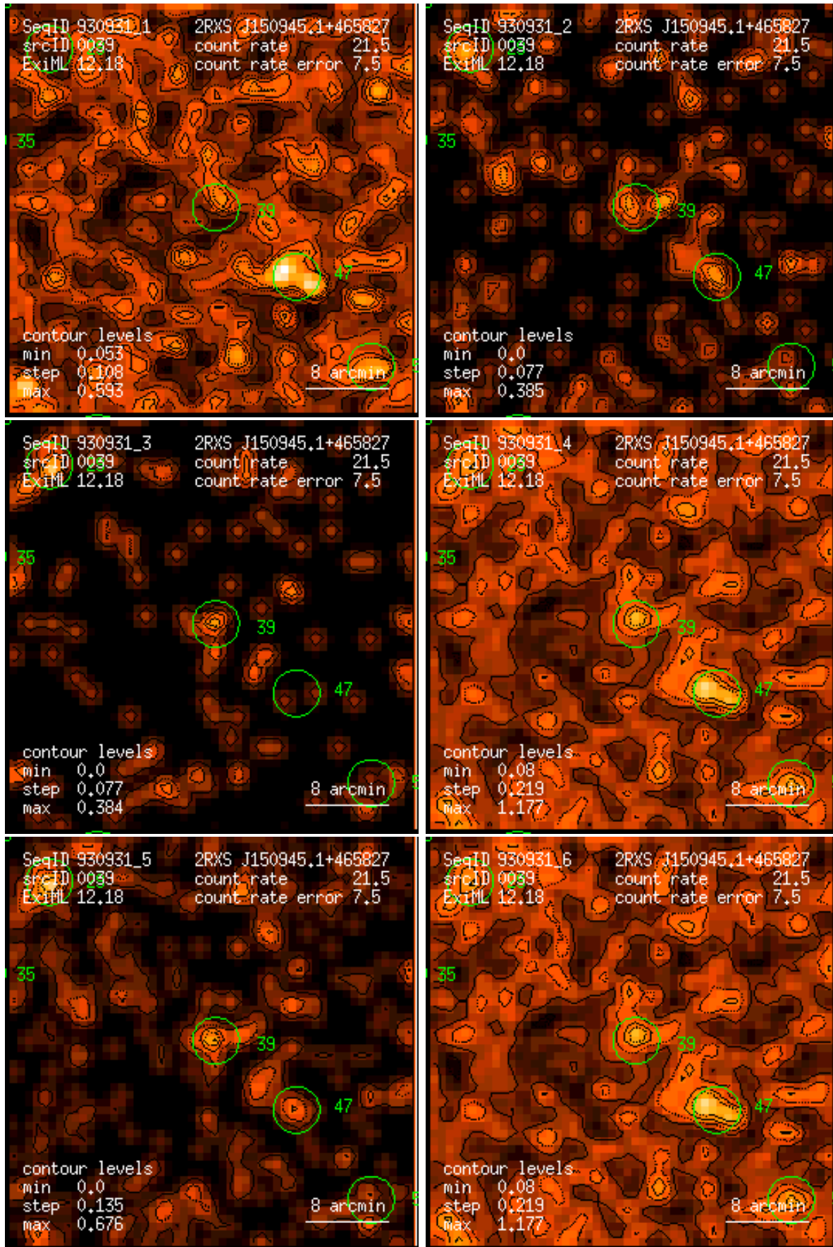
Figure 39: RASS 930931: detection 0039: band rate images, Gaussian filter: (1) PSPC channels 11 – 41, (2) 52 – 90, (3) 91 – 201, (4) 11 – 235, (5) 52 – 201, (6) 11 – 201. Broad band rates in counts/ks. Band rate contour levels in counts/ks/arcmin 2 .
