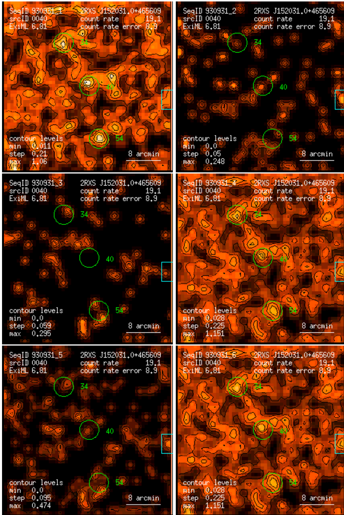
Figure 40: RASS 930931: detection 0040: band rate images, Gaussian filter: (1) PSPC channels 11 – 41, (2) 52 – 90, (3) 91 – 201, (4) 11 – 235, (5) 52 – 201, (6) 11 – 201. Broad band rates in counts/ks. Band rate contour levels in counts/ks/arcmin 2 .
