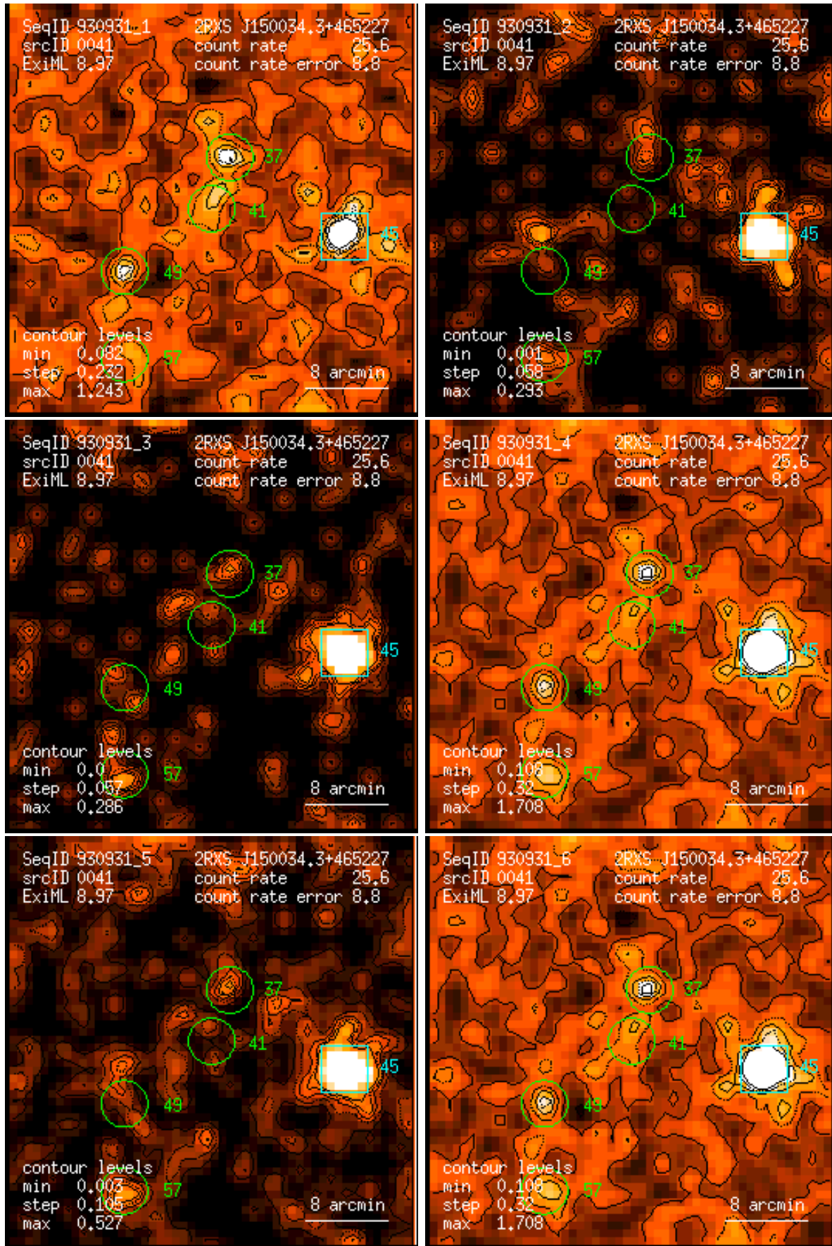
Figure 41: RASS 930931: detection 0041: band rate images, Gaussian filter: (1) PSPC channels 11 – 41, (2) 52 – 90, (3) 91 – 201, (4) 11 – 235, (5) 52 – 201, (6) 11 – 201. Broad band rates in counts/ks. Band rate contour levels in counts/ks/arcmin 2 .
