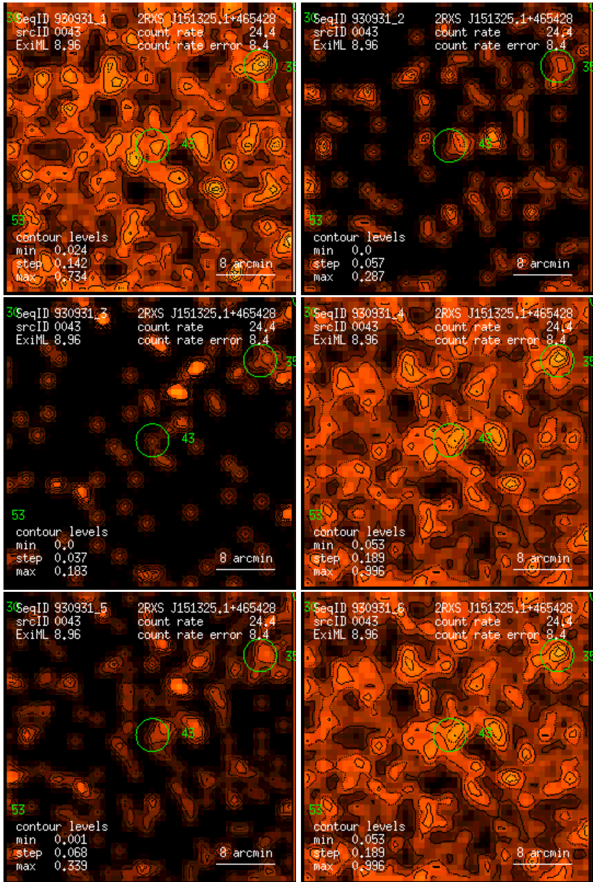
Figure 43: RASS 930931: detection 0043: band rate images, Gaussian filter: (1) PSPC channels 11 – 41, (2) 52 – 90, (3) 91 – 201, (4) 11 – 235, (5) 52 – 201, (6) 11 – 201. Broad band rates in counts/ks. Band rate contour levels in counts/ks/arcmin 2 .
