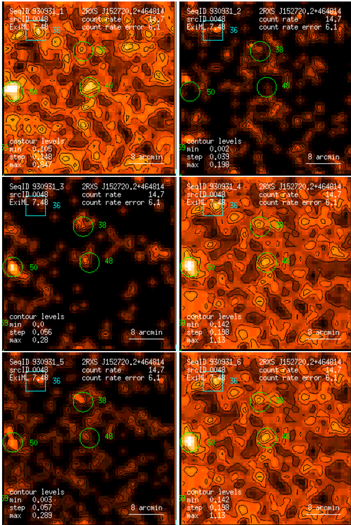
Figure 48: RASS 930931: detection 0048: band rate images, Gaussian filter: (1) PSPC channels 11 – 41, (2) 52 – 90, (3) 91 – 201, (4) 11 – 235, (5) 52 – 201, (6) 11 – 201. Broad band rates in counts/ks. Band rate contour levels in counts/ks/arcmin 2 .
