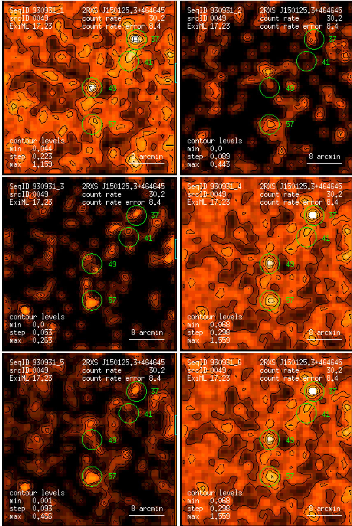
Figure 49: RASS 930931: detection 0049: band rate images, Gaussian filter: (1) PSPC channels 11 – 41, (2) 52 – 90, (3) 91 – 201, (4) 11 – 235, (5) 52 – 201, (6) 11 – 201. Broad band rates in counts/ks. Band rate contour levels in counts/ks/arcmin 2 .
