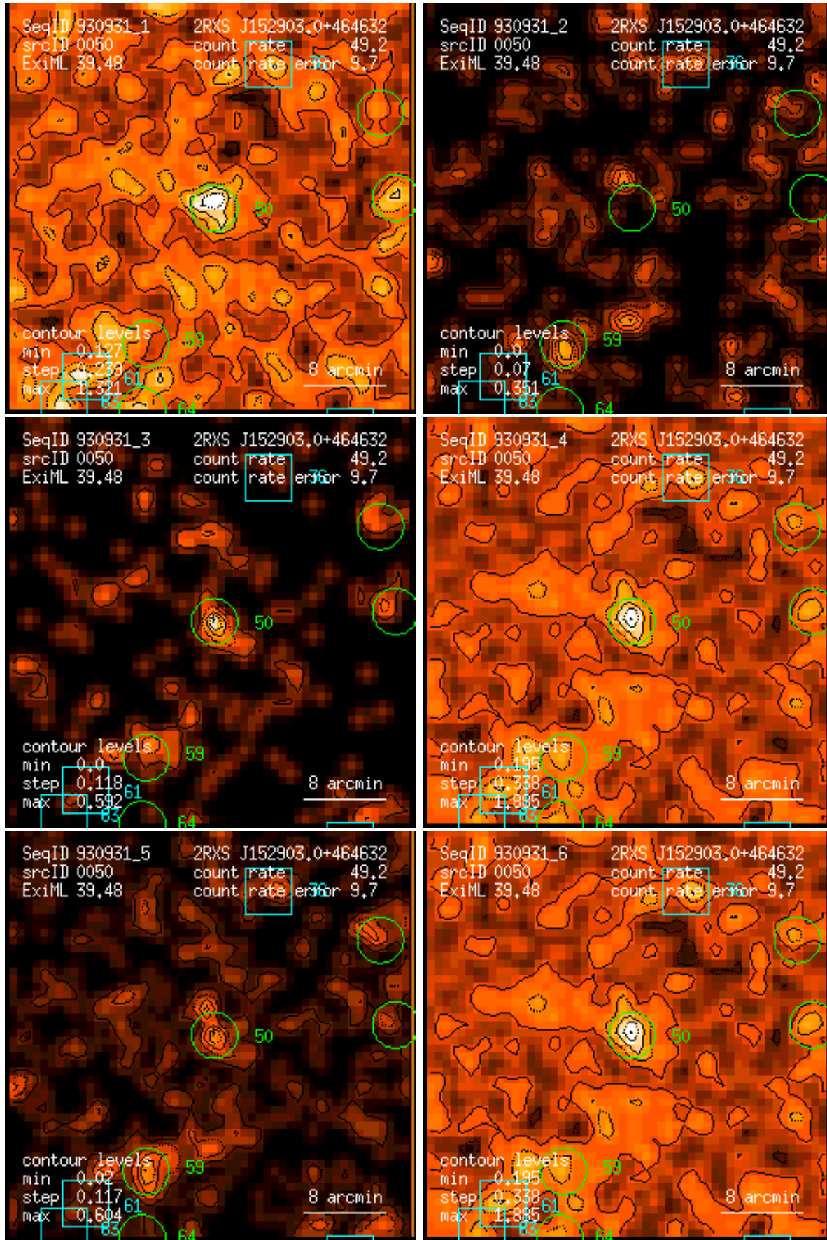
Figure 50: RASS 930931: detection 0050: band rate images, Gaussian filter: (1) PSPC channels 11 – 41, (2) 52 – 90, (3) 91 – 201, (4) 11 – 235, (5) 52 – 201, (6) 11 – 201. Broad band rates in counts/ks. Band rate contour levels in counts/ks/arcmin 2 .
