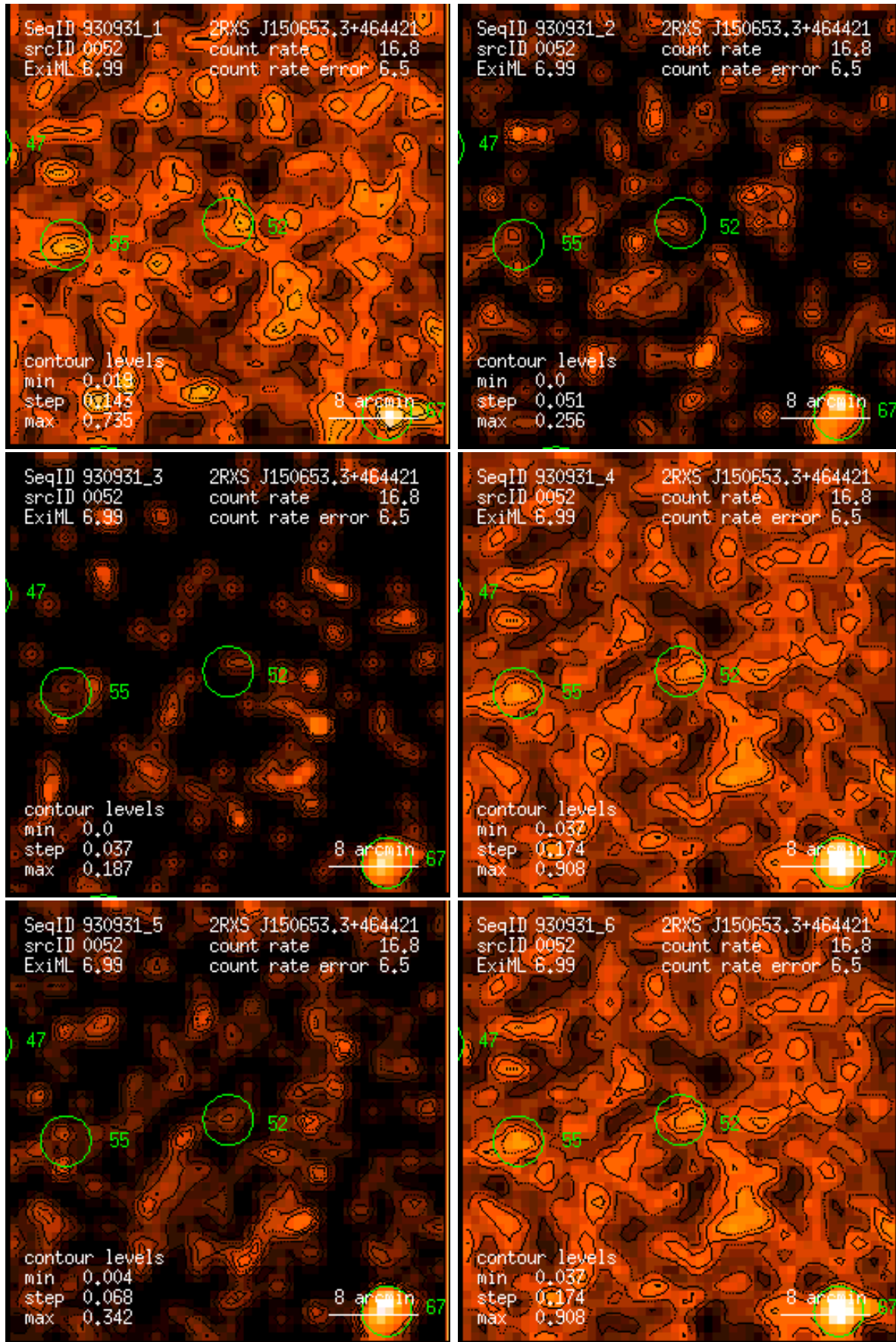
Figure 52: RASS 930931: detection 0052: band rate images, Gaussian filter: (1) PSPC channels 11 – 41, (2) 52 – 90, (3) 91 – 201, (4) 11 – 235, (5) 52 – 201, (6) 11 – 201. Broad band rates in counts/ks. Band rate contour levels in counts/ks/arcmin 2 .
