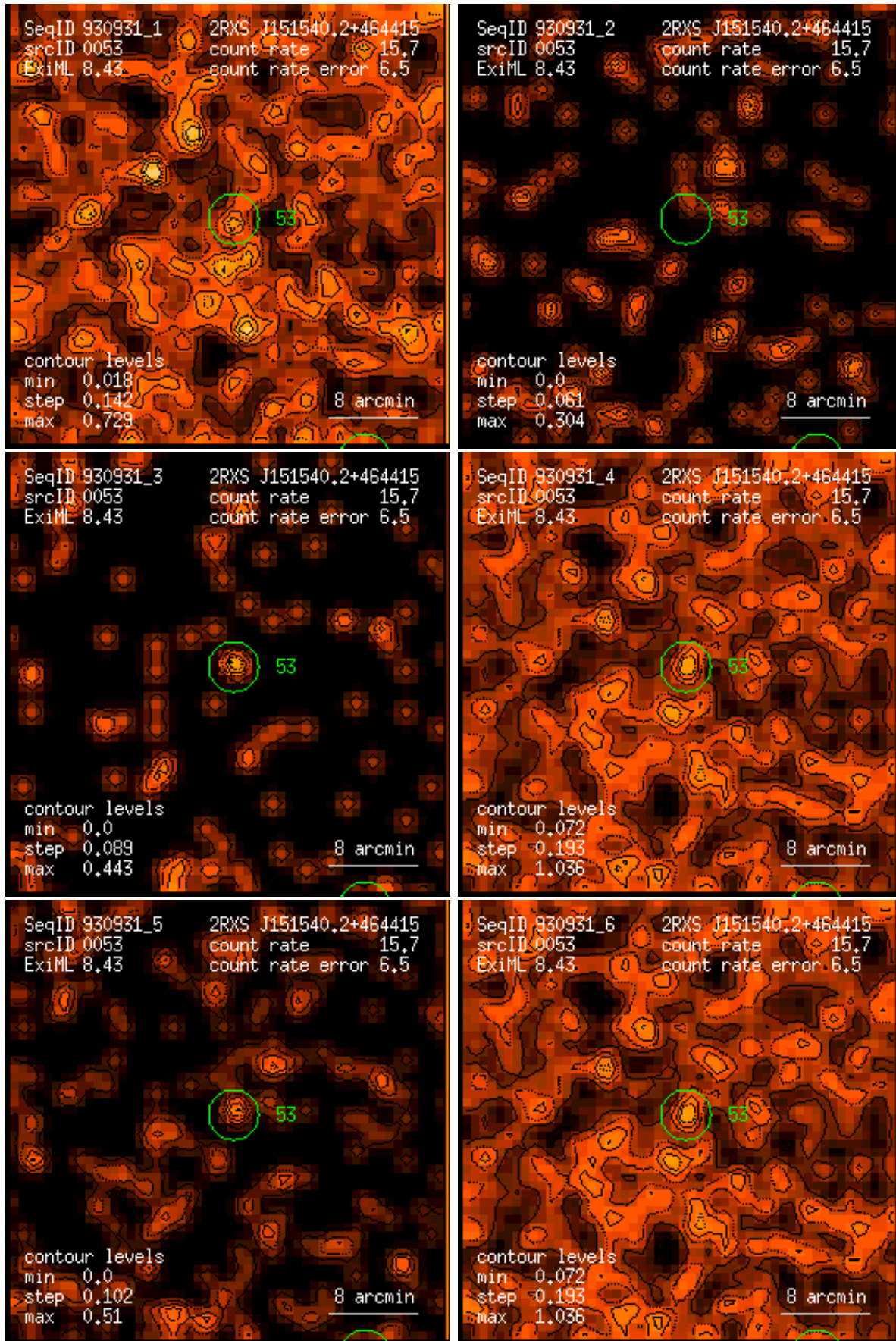
Figure 53: RASS 930931: detection 0053: band rate images, Gaussian filter: (1) PSPC channels 11 – 41, (2) 52 – 90, (3) 91 – 201, (4) 11 – 235, (5) 52 – 201, (6) 11 – 201. Broad band rates in counts/ks. Band rate contour levels in counts/ks/arcmin 2 .
