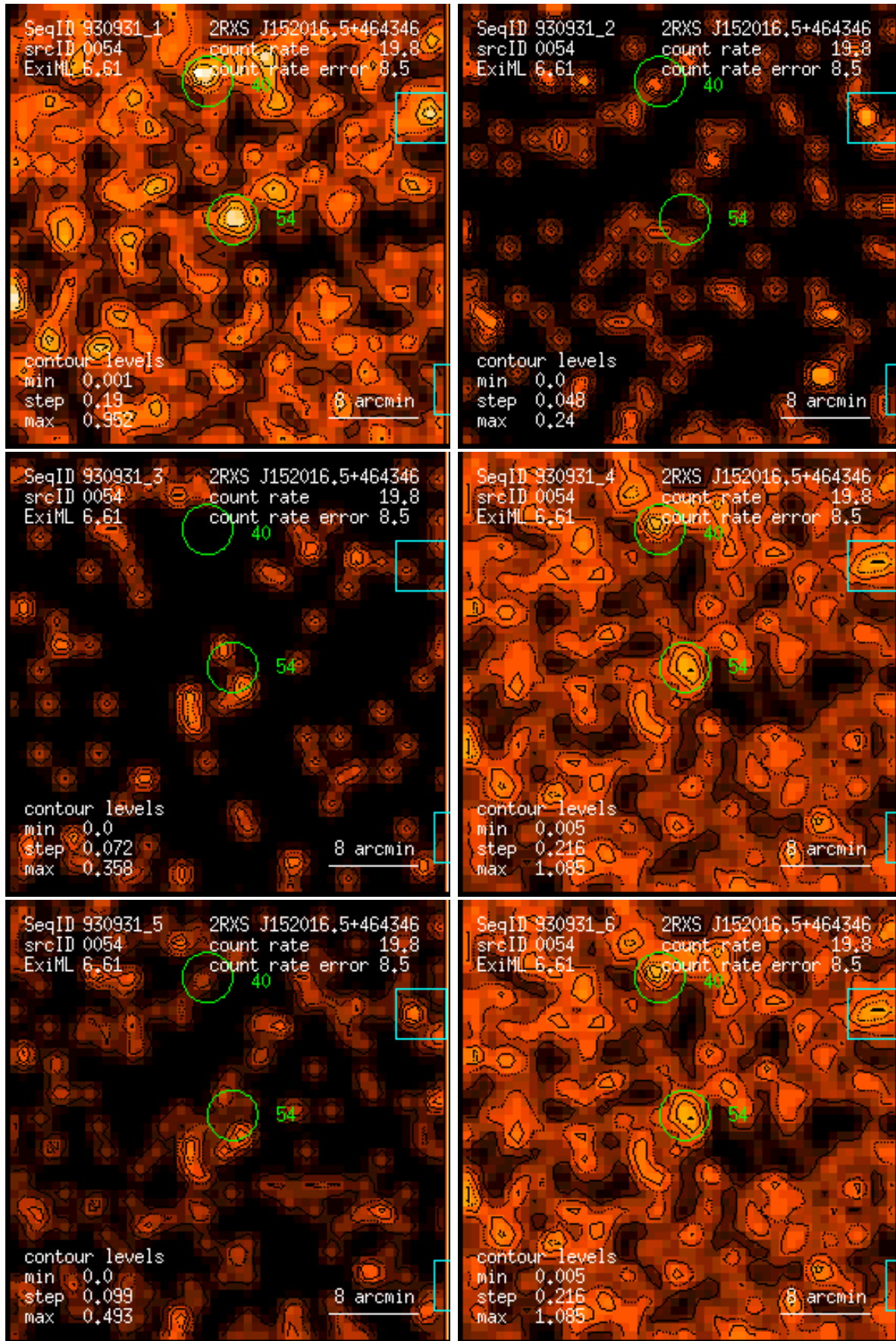
Figure 54: RASS 930931: detection 0054: band rate images, Gaussian filter: (1) PSPC channels 11 – 41, (2) 52 – 90, (3) 91 – 201, (4) 11 – 235, (5) 52 – 201, (6) 11 – 201. Broad band rates in counts/ks. Band rate contour levels in counts/ks/arcmin 2 .
