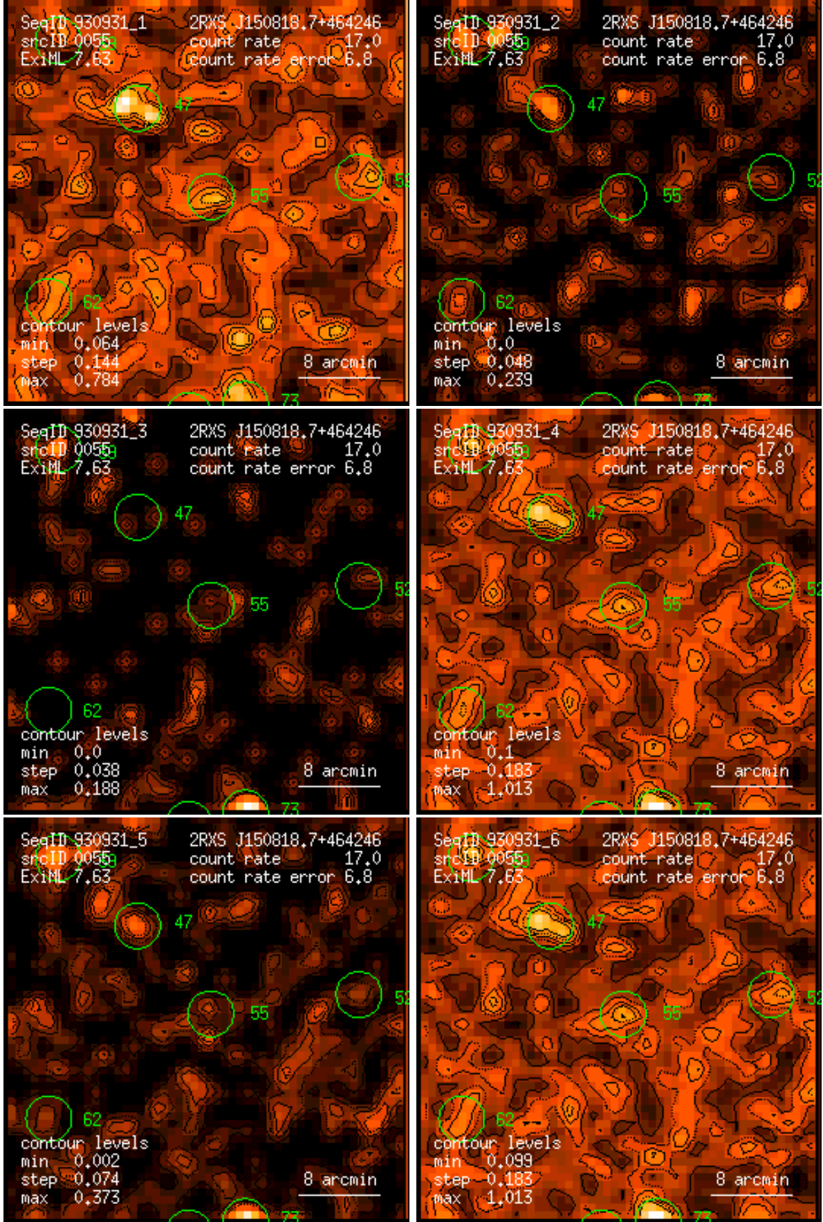
Figure 55: RASS 930931: detection 0055: band rate images, Gaussian filter: (1) PSPC channels 11 – 41, (2) 52 – 90, (3) 91 – 201, (4) 11 – 235, (5) 52 – 201, (6) 11 – 201. Broad band rates in counts/ks. Band rate contour levels in counts/ks/arcmin 2 .
