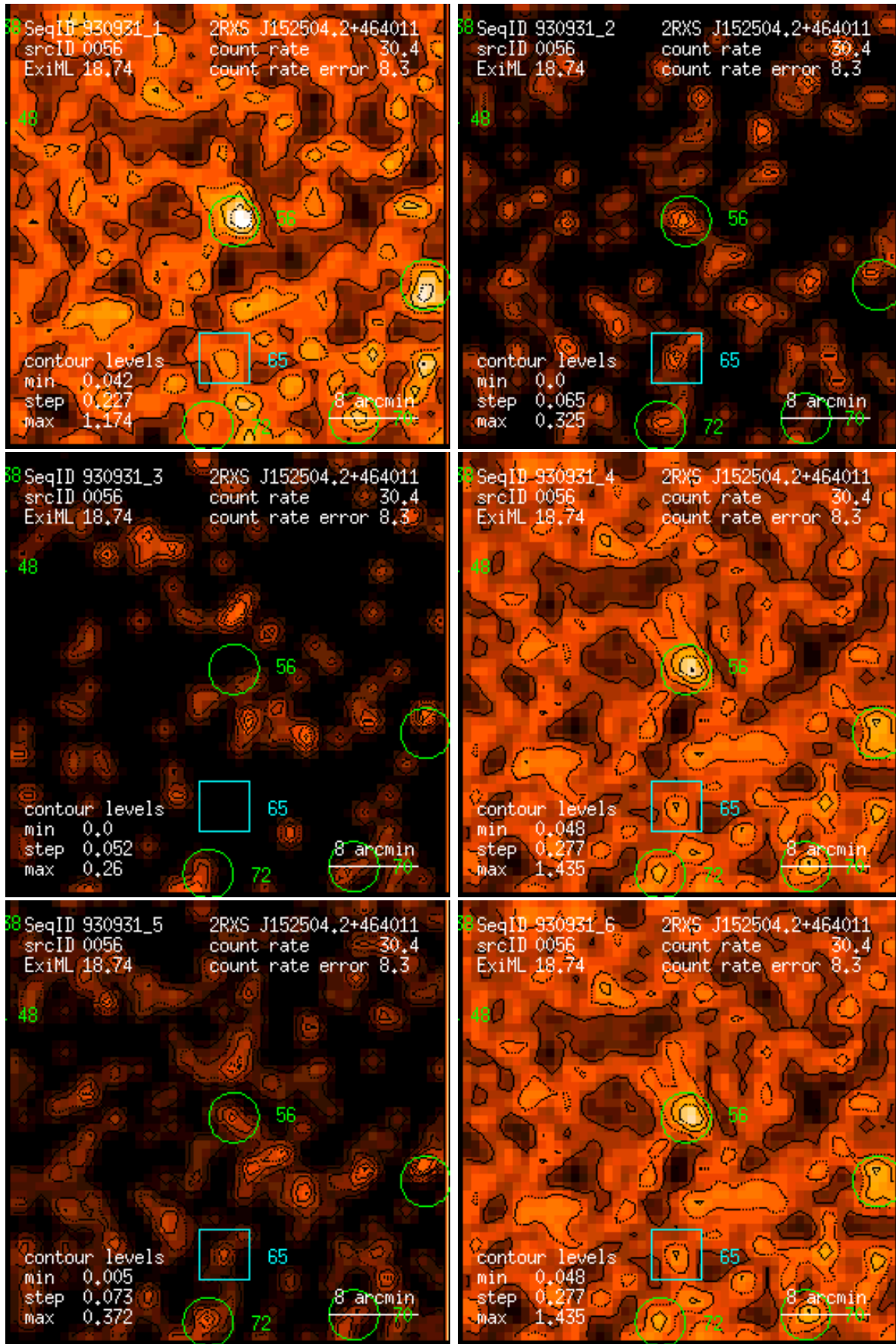
Figure 56: RASS 930931: detection 0056: band rate images, Gaussian filter: (1) PSPC channels 11 – 41, (2) 52 – 90, (3) 91 – 201, (4) 11 – 235, (5) 52 – 201, (6) 11 – 201. Broad band rates in counts/ks. Band rate contour levels in counts/ks/arcmin 2 .
