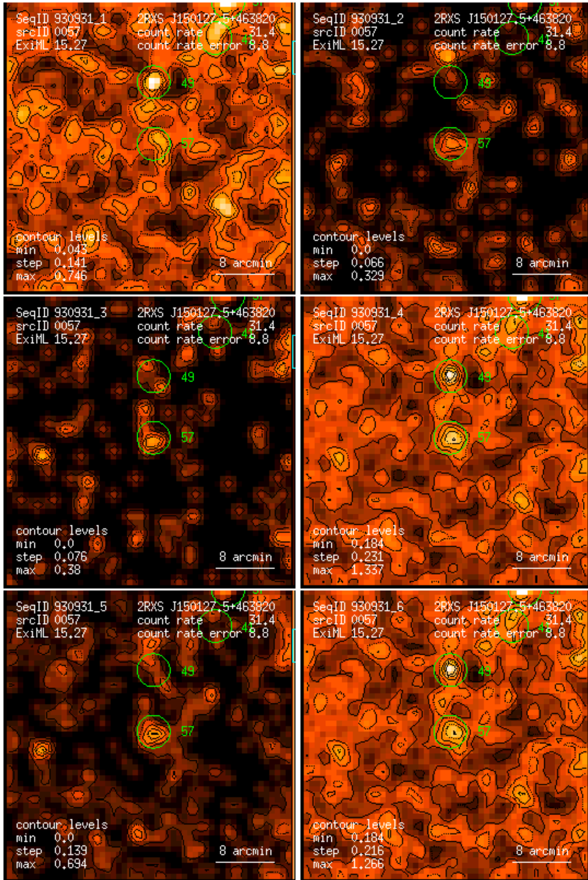
Figure 57: RASS 930931: detection 0057: band rate images, Gaussian filter: (1) PSPC channels 11 – 41, (2) 52 – 90, (3) 91 – 201, (4) 11 – 235, (5) 52 – 201, (6) 11 – 201. Broad band rates in counts/ks. Band rate contour levels in counts/ks/arcmin 2 .
