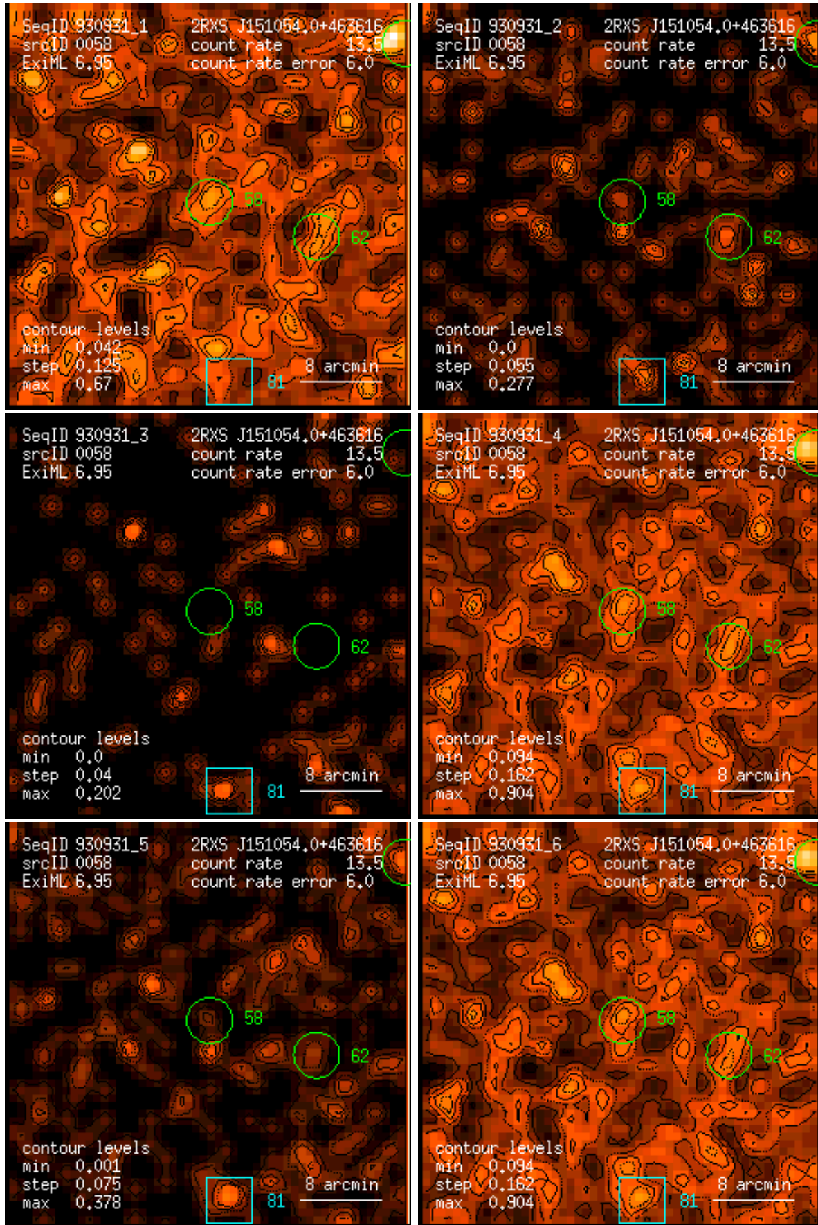
Figure 58: RASS 930931: detection 0058: band rate images, Gaussian filter: (1) PSPC channels 11 – 41, (2) 52 – 90, (3) 91 – 201, (4) 11 – 235, (5) 52 – 201, (6) 11 – 201. Broad band rates in counts/ks. Band rate contour levels in counts/ks/arcmin 2 .
