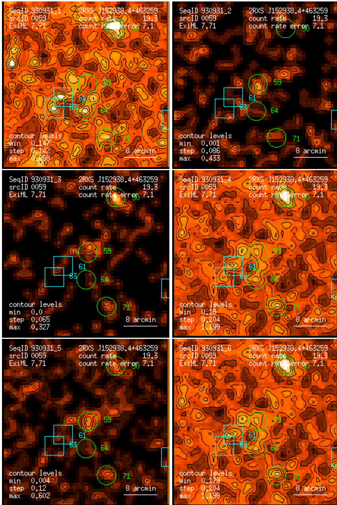
Figure 59: RASS 930931: detection 0059: band rate images, Gaussian filter: (1) PSPC channels 11 – 41, (2) 52 – 90, (3) 91 – 201, (4) 11 – 235, (5) 52 – 201, (6) 11 – 201. Broad band rates in counts/ks. Band rate contour levels in counts/ks/arcmin 2 .
