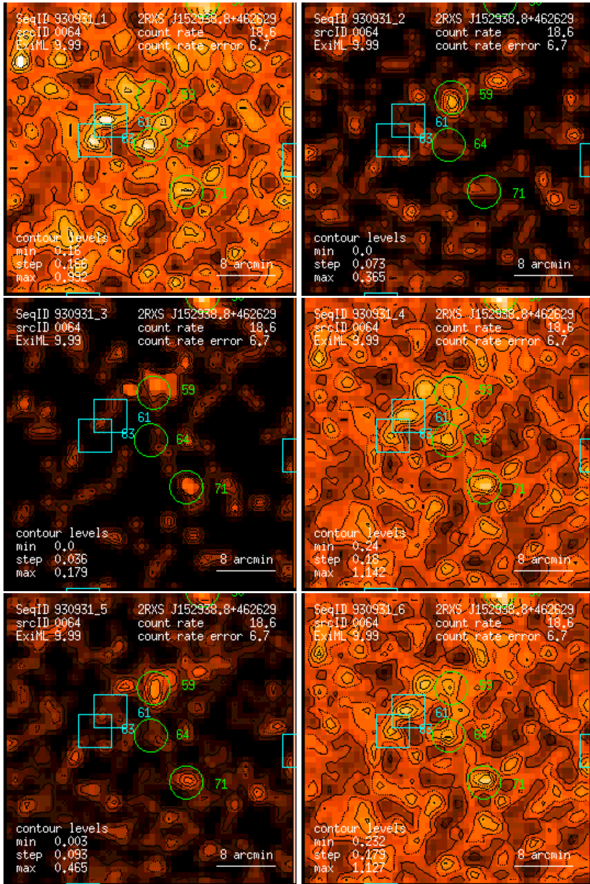
Figure 64: RASS 930931: detection 0064: band rate images, Gaussian filter: (1) PSPC channels 11 – 41, (2) 52 – 90, (3) 91 – 201, (4) 11 – 235, (5) 52 – 201, (6) 11 – 201. Broad band rates in counts/ks. Band rate contour levels in counts/ks/arcmin 2 .
