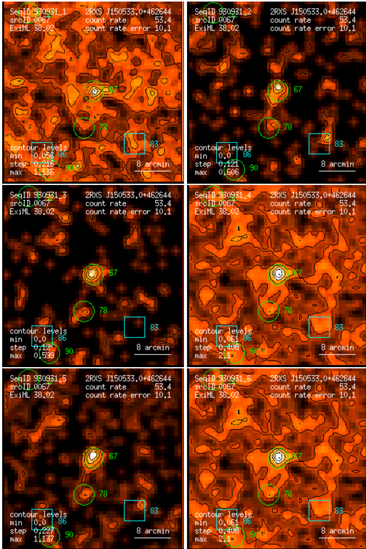
Figure 67: RASS 930931: detection 0067: band rate images, Gaussian filter: (1) PSPC channels 11 – 41, (2) 52 – 90, (3) 91 – 201, (4) 11 – 235, (5) 52 – 201, (6) 11 – 201. Broad band rates in counts/ks. Band rate contour levels in counts/ks/arcmin 2 .
