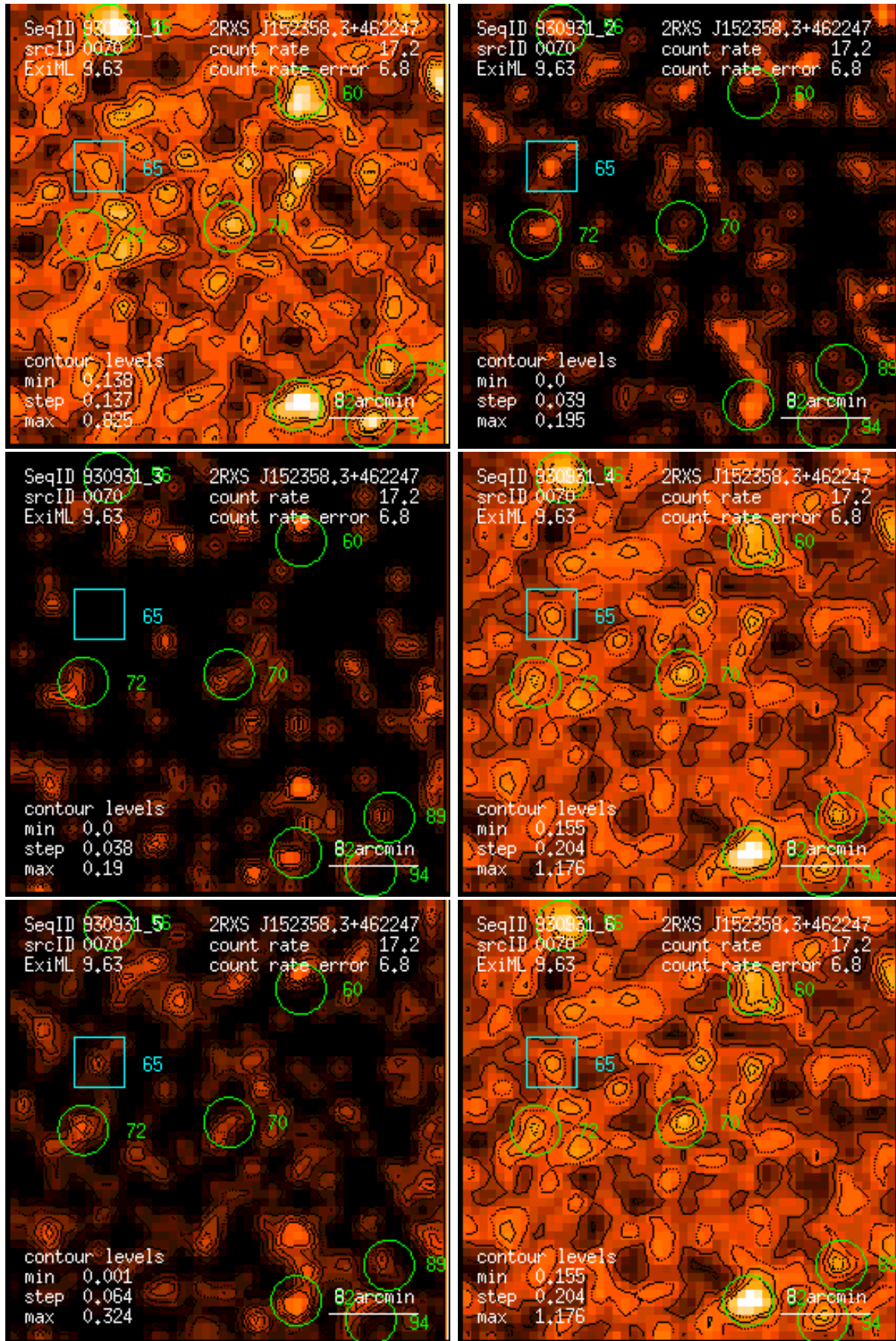
Figure 70: RASS 930931: detection 0070: band rate images, Gaussian filter: (1) PSPC channels 11 – 41, (2) 52 – 90, (3) 91 – 201, (4) 11 – 235, (5) 52 – 201, (6) 11 – 201. Broad band rates in counts/ks. Band rate contour levels in counts/ks/arcmin 2 .
