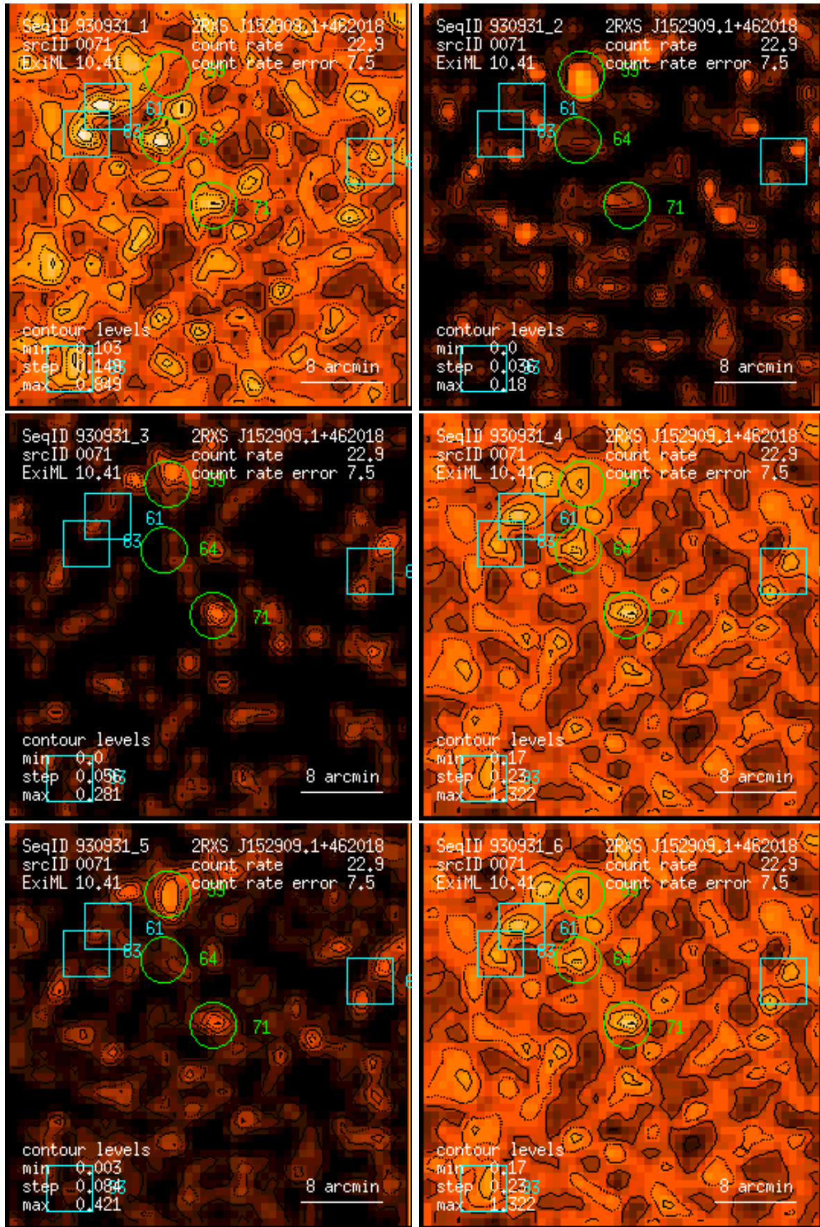
Figure 71: RASS 930931: detection 0071: band rate images, Gaussian filter: (1) PSPC channels 11 – 41, (2) 52 – 90, (3) 91 – 201, (4) 11 – 235, (5) 52 – 201, (6) 11 – 201. Broad band rates in counts/ks. Band rate contour levels in counts/ks/arcmin 2 .
