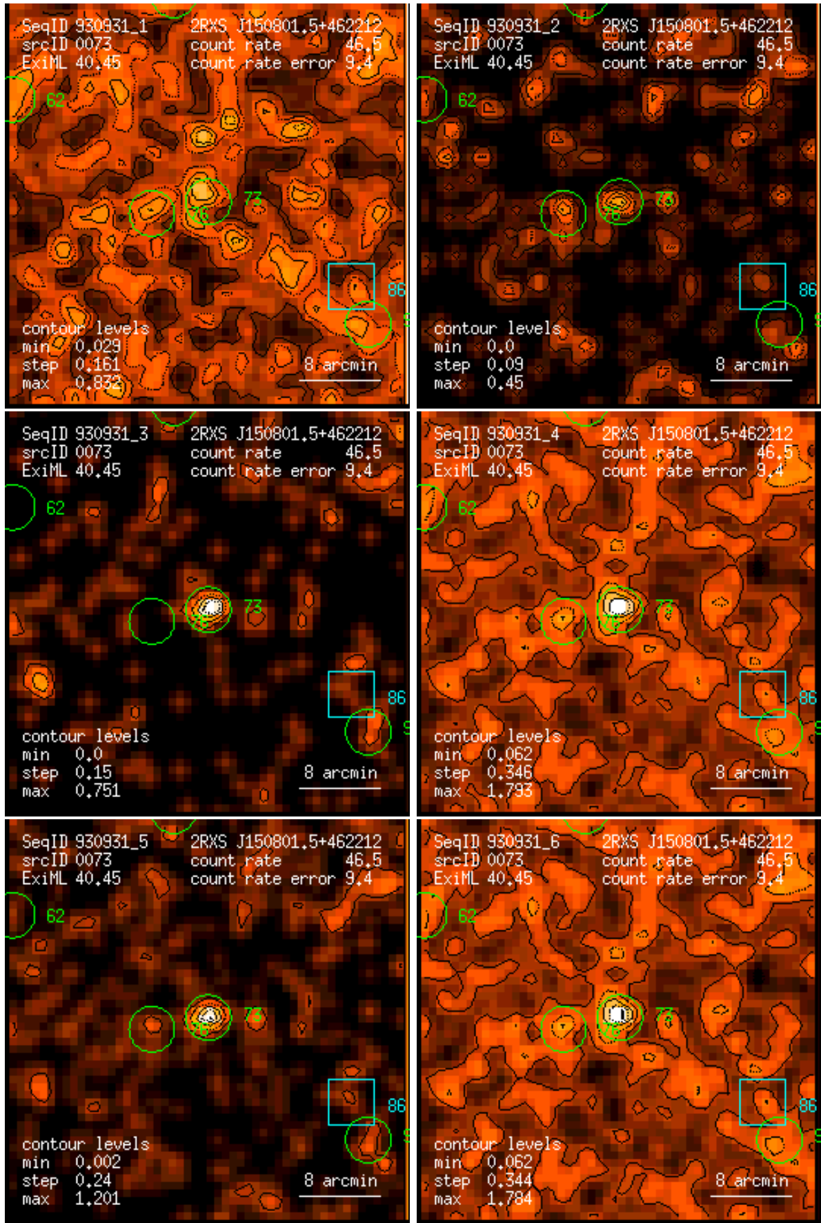
Figure 73: RASS 930931: detection 0073: band rate images, Gaussian filter: (1) PSPC channels 11 – 41, (2) 52 – 90, (3) 91 – 201, (4) 11 – 235, (5) 52 – 201, (6) 11 – 201. Broad band rates in counts/ks. Band rate contour levels in counts/ks/arcmin 2 .
