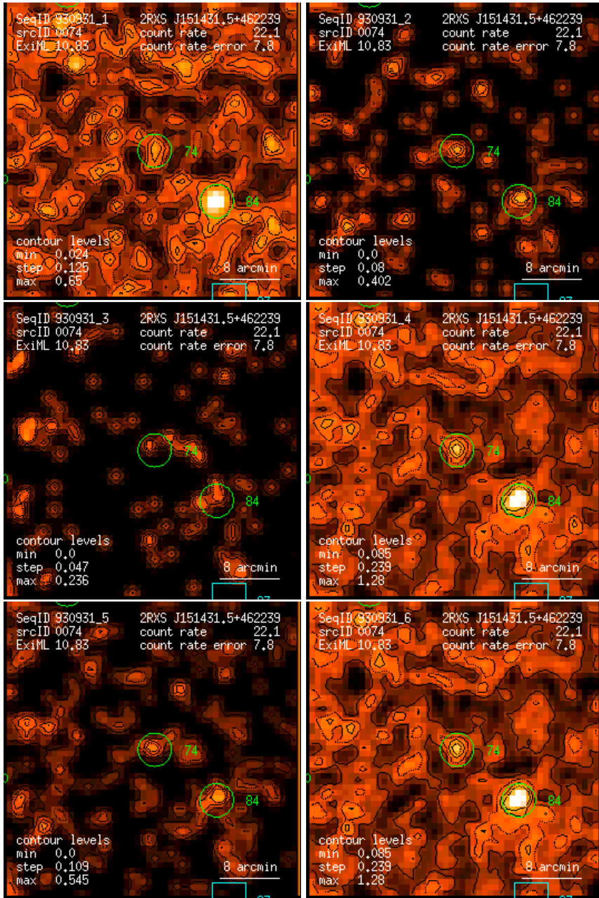
Figure 74: RASS 930931: detection 0074: band rate images, Gaussian filter: (1) PSPC channels 11 – 41, (2) 52 – 90, (3) 91 – 201, (4) 11 – 235, (5) 52 – 201, (6) 11 – 201. Broad band rates in counts/ks. Band rate contour levels in counts/ks/arcmin 2 .
