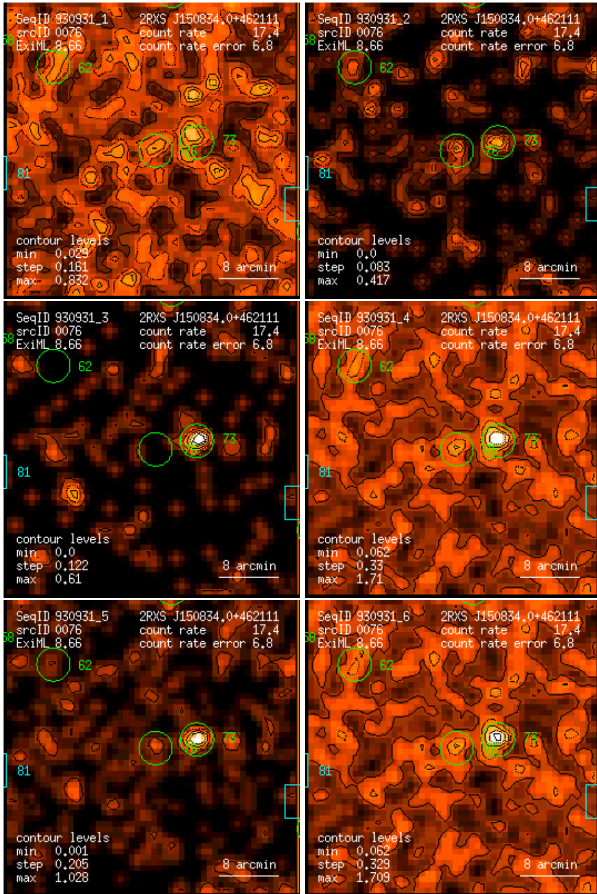
Figure 76: RASS 930931: detection 0076: band rate images, Gaussian filter: (1) PSPC channels 11 – 41, (2) 52 – 90, (3) 91 – 201, (4) 11 – 235, (5) 52 – 201, (6) 11 – 201. Broad band rates in counts/ks. Band rate contour levels in counts/ks/arcmin 2 .
