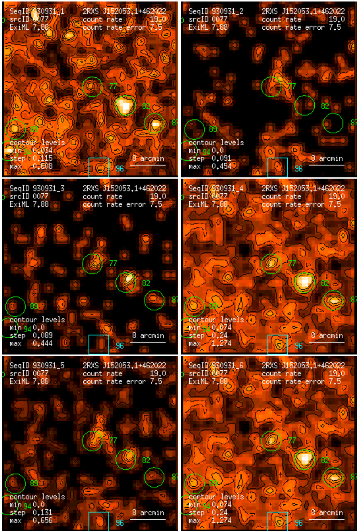
Figure 77: RASS 930931: detection 0077: band rate images, Gaussian filter: (1) PSPC channels 11 – 41, (2) 52 – 90, (3) 91 – 201, (4) 11 – 235, (5) 52 – 201, (6) 11 – 201. Broad band rates in counts/ks. Band rate contour levels in counts/ks/arcmin 2 .
