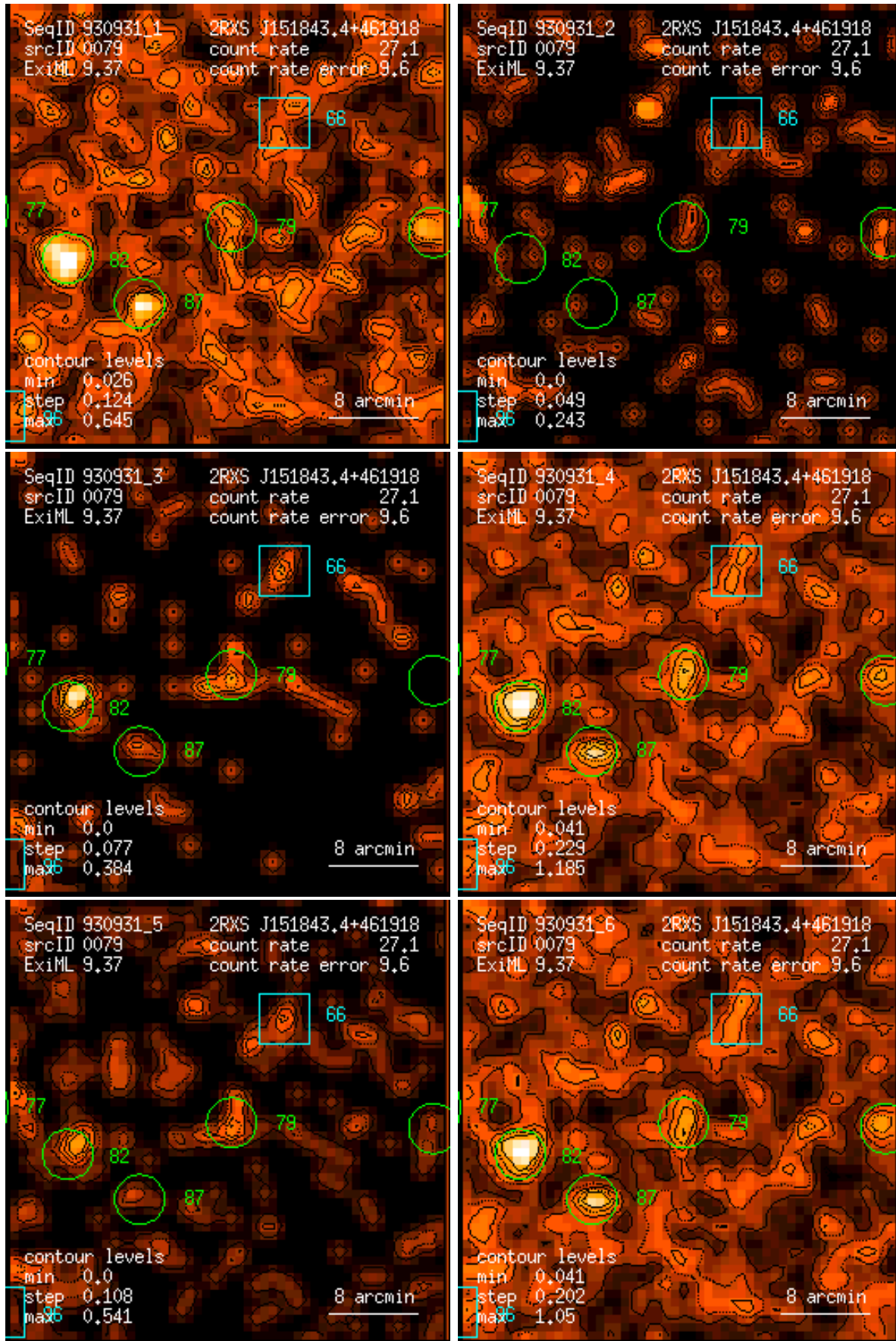
Figure 79: RASS 930931: detection 0079: band rate images, Gaussian filter: (1) PSPC channels 11 – 41, (2) 52 – 90, (3) 91 – 201, (4) 11 – 235, (5) 52 – 201, (6) 11 – 201. Broad band rates in counts/ks. Band rate contour levels in counts/ks/arcmin 2 .
