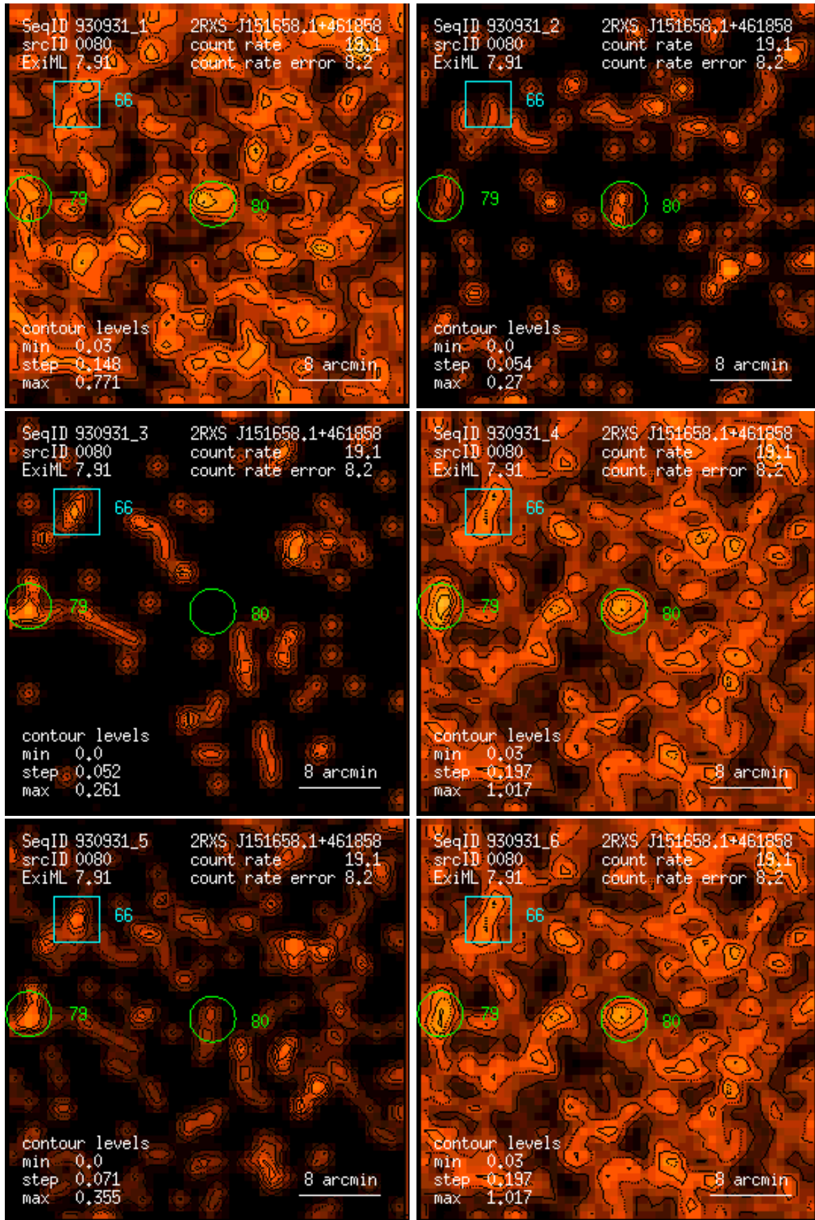
Figure 80: RASS 930931: detection 0080: band rate images, Gaussian filter: (1) PSPC channels 11 – 41, (2) 52 – 90, (3) 91 – 201, (4) 11 – 235, (5) 52 – 201, (6) 11 – 201. Broad band rates in counts/ks. Band rate contour levels in counts/ks/arcmin 2 .
