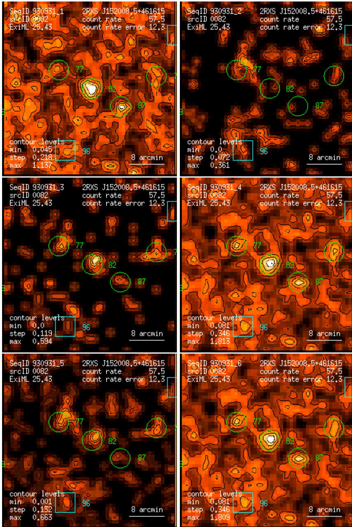
Figure 82: RASS 930931: detection 0082: band rate images, Gaussian filter: (1) PSPC channels 11 – 41, (2) 52 – 90, (3) 91 – 201, (4) 11 – 235, (5) 52 – 201, (6) 11 – 201. Broad band rates in counts/ks. Band rate contour levels in counts/ks/arcmin 2 .
