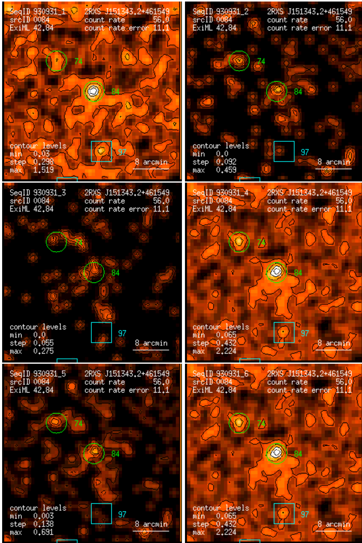
Figure 84: RASS 930931: detection 0084: band rate images, Gaussian filter: (1) PSPC channels 11 – 41, (2) 52 – 90, (3) 91 – 201, (4) 11 – 235, (5) 52 – 201, (6) 11 – 201. Broad band rates in counts/ks. Band rate contour levels in counts/ks/arcmin 2 .
