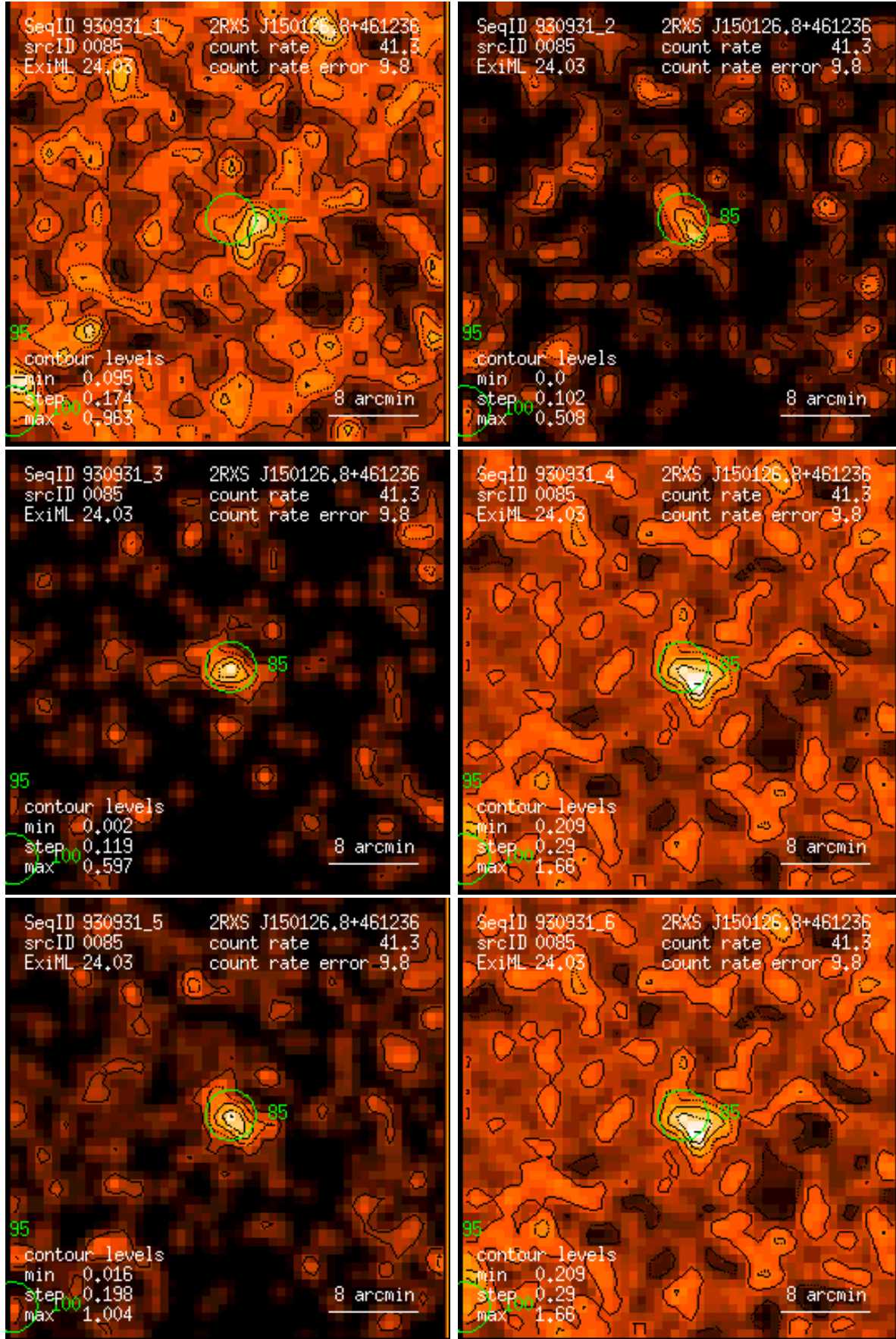
Figure 85: RASS 930931: detection 0085: band rate images, Gaussian filter: (1) PSPC channels 11 – 41, (2) 52 – 90, (3) 91 – 201, (4) 11 – 235, (5) 52 – 201, (6) 11 – 201. Broad band rates in counts/ks. Band rate contour levels in counts/ks/arcmin 2 .
