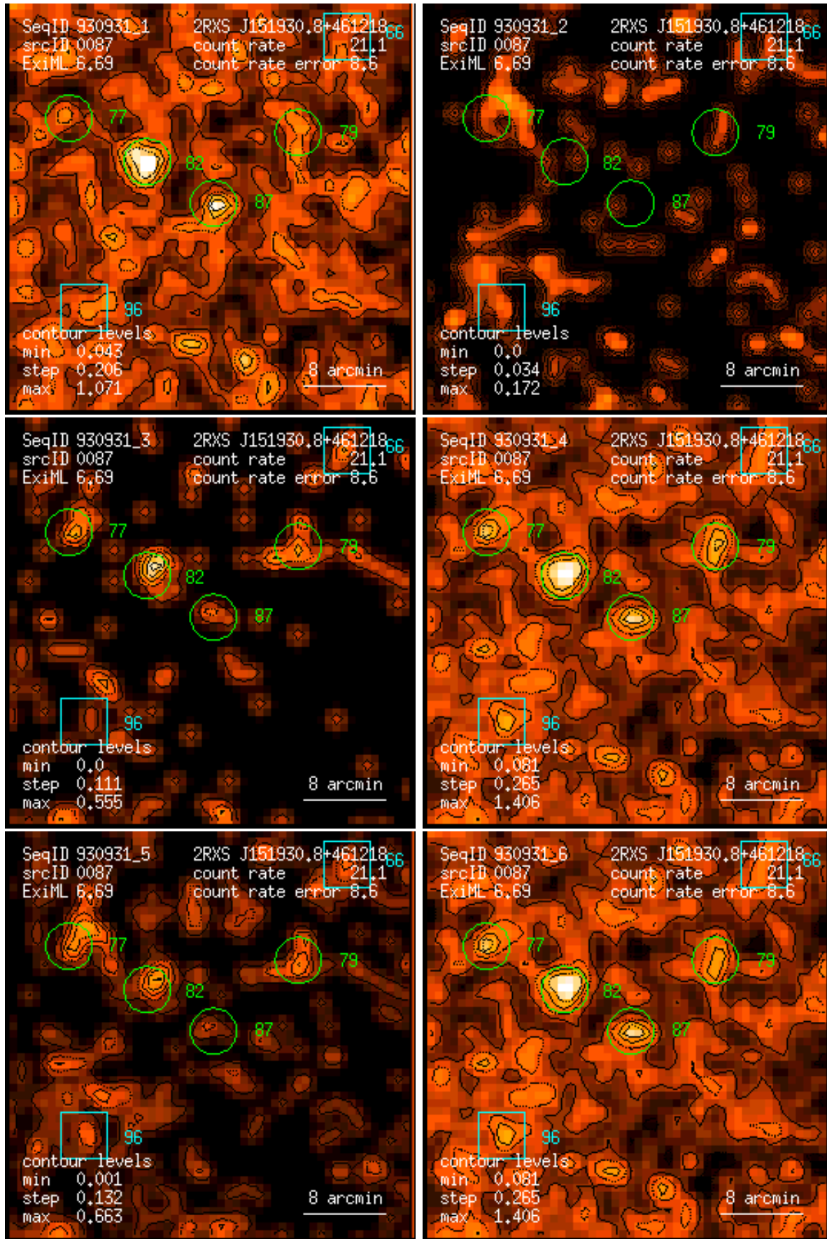
Figure 87: RASS 930931: detection 0087: band rate images, Gaussian filter: (1) PSPC channels 11 – 41, (2) 52 – 90, (3) 91 – 201, (4) 11 – 235, (5) 52 – 201, (6) 11 – 201. Broad band rates in counts/ks. Band rate contour levels in counts/ks/arcmin 2 .
