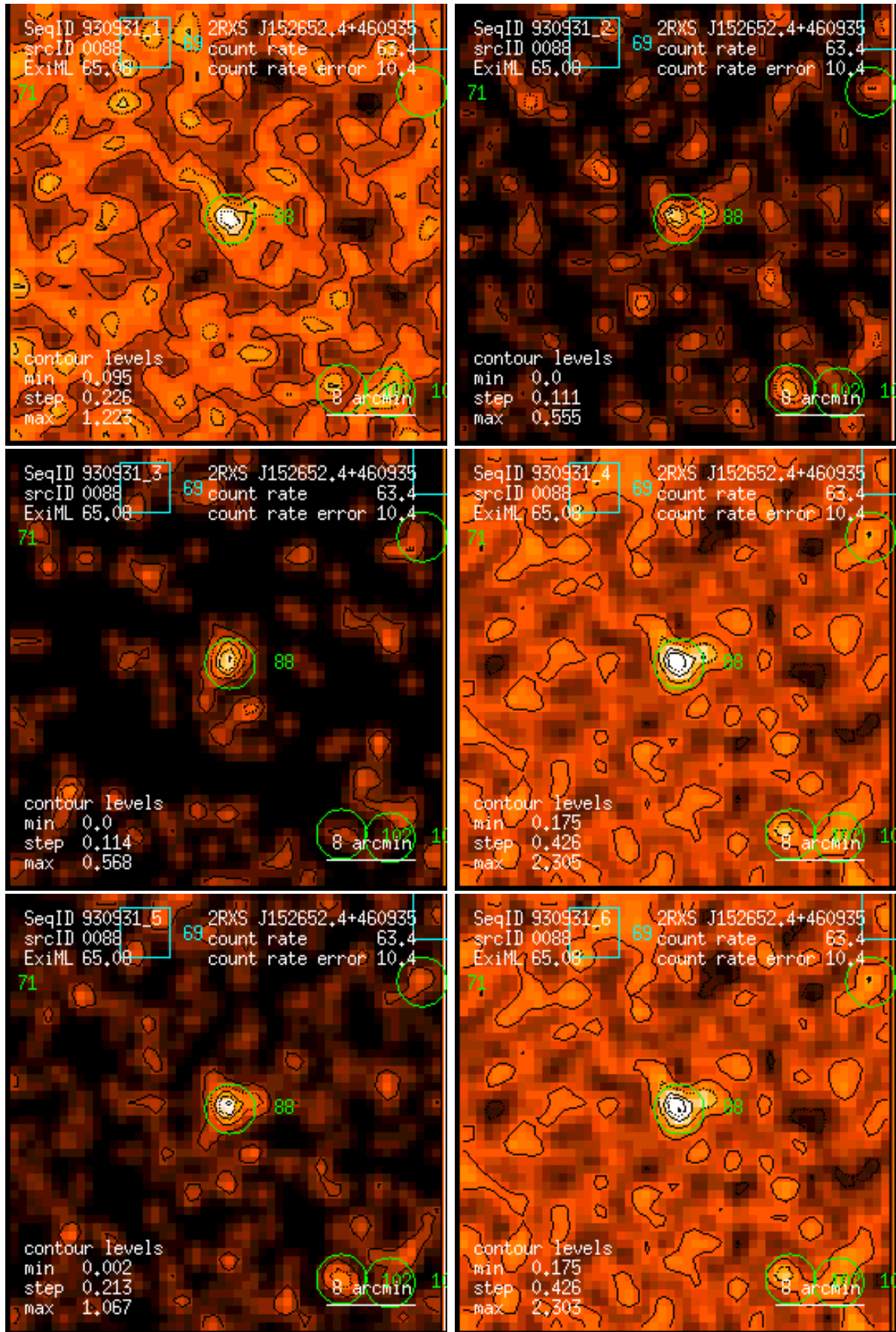
Figure 88: RASS 930931: detection 0088: band rate images, Gaussian filter: (1) PSPC channels 11 – 41, (2) 52 – 90, (3) 91 – 201, (4) 11 – 235, (5) 52 – 201, (6) 11 – 201. Broad band rates in counts/ks. Band rate contour levels in counts/ks/arcmin 2 .
