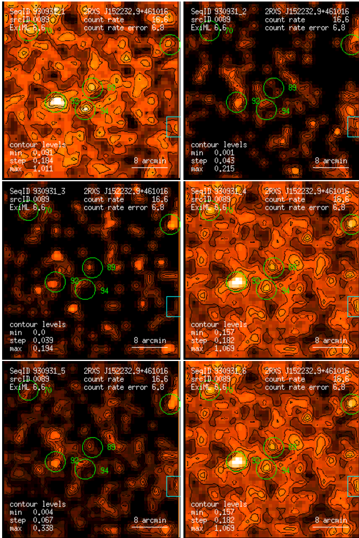
Figure 89: RASS 930931: detection 0089: band rate images, Gaussian filter: (1) PSPC channels 11 – 41, (2) 52 – 90, (3) 91 – 201, (4) 11 – 235, (5) 52 – 201, (6) 11 – 201. Broad band rates in counts/ks. Band rate contour levels in counts/ks/arcmin 2 .
