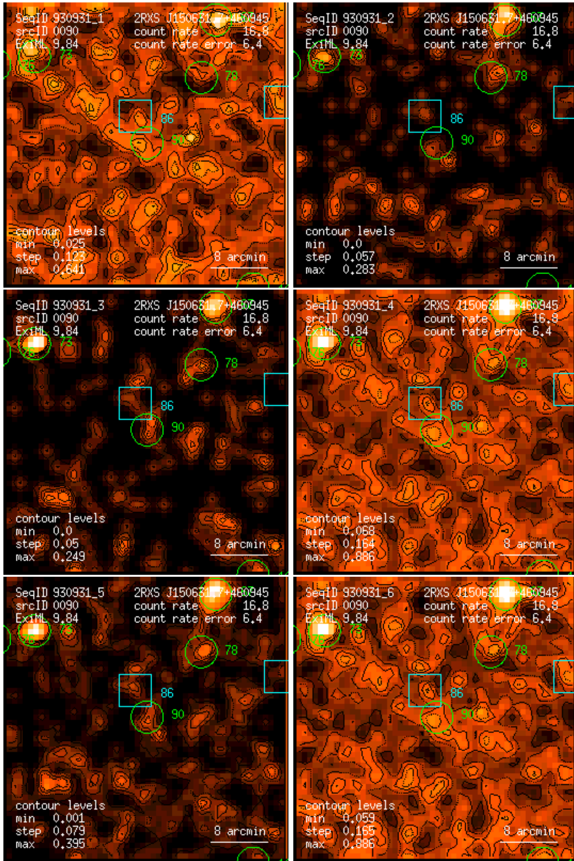
Figure 90: RASS 930931: detection 0090: band rate images, Gaussian filter: (1) PSPC channels 11 – 41, (2) 52 – 90, (3) 91 – 201, (4) 11 – 235, (5) 52 – 201, (6) 11 – 201. Broad band rates in counts/ks. Band rate contour levels in counts/ks/arcmin 2 .
