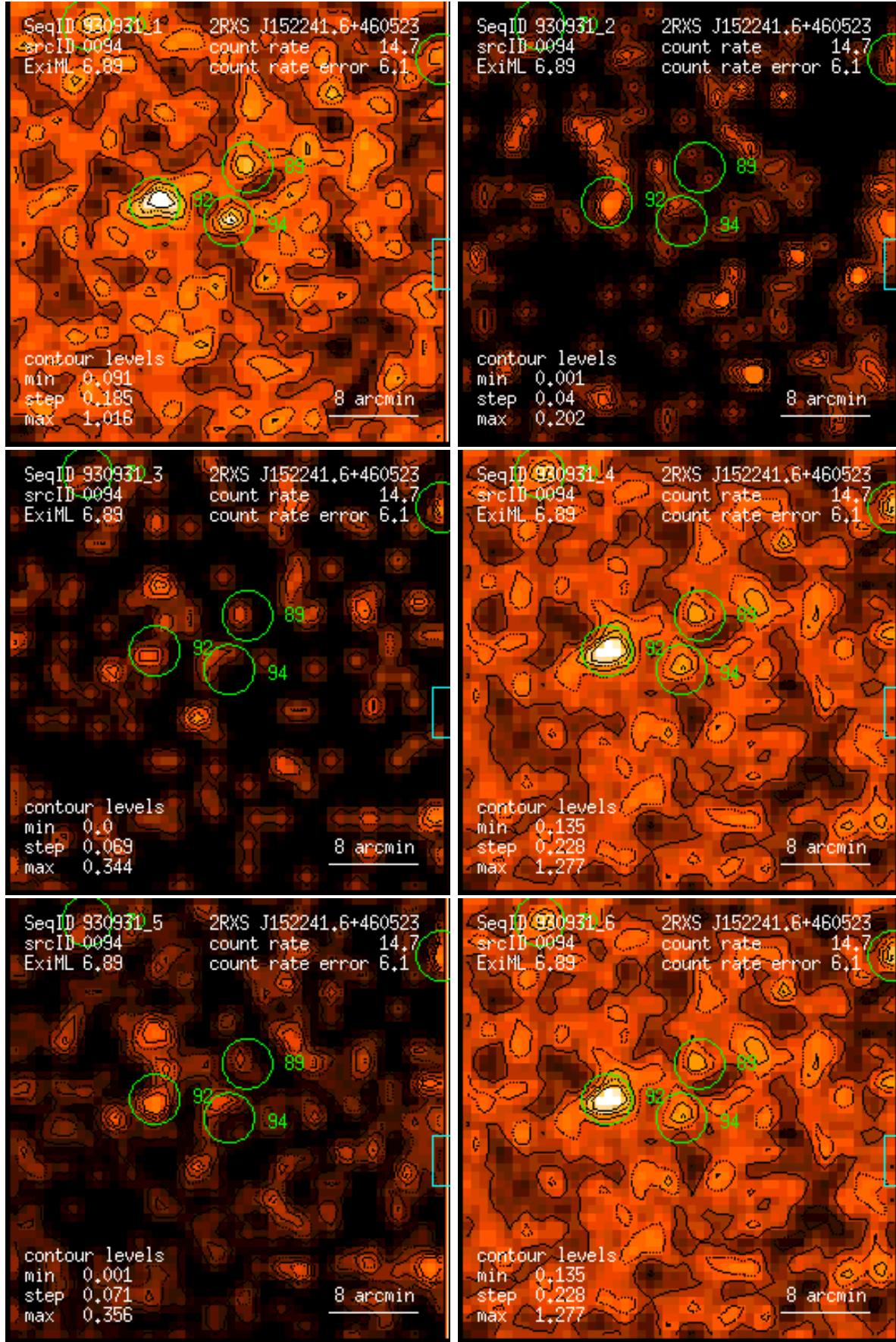
Figure 94: RASS 930931: detection 0094: band rate images, Gaussian filter: (1) PSPC channels 11 – 41, (2) 52 – 90, (3) 91 – 201, (4) 11 – 235, (5) 52 – 201, (6) 11 – 201. Broad band rates in counts/ks. Band rate contour levels in counts/ks/arcmin 2 .
