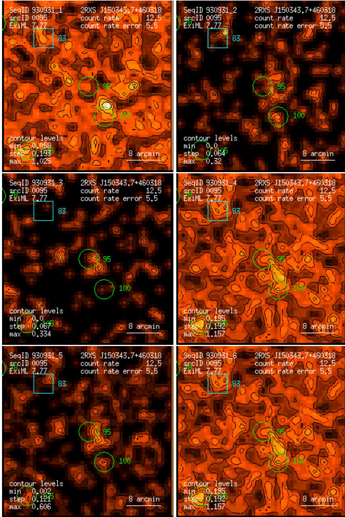
Figure 95: RASS 930931: detection 0095: band rate images, Gaussian filter: (1) PSPC channels 11 – 41, (2) 52 – 90, (3) 91 – 201, (4) 11 – 235, (5) 52 – 201, (6) 11 – 201. Broad band rates in counts/ks. Band rate contour levels in counts/ks/arcmin 2 .
