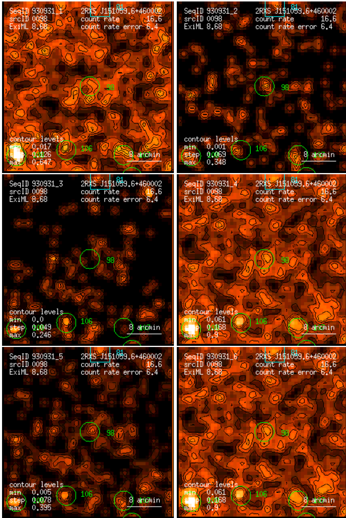
Figure 98: RASS 930931: detection 0098: band rate images, Gaussian filter: (1) PSPC channels 11 – 41, (2) 52 – 90, (3) 91 – 201, (4) 11 – 235, (5) 52 – 201, (6) 11 – 201. Broad band rates in counts/ks. Band rate contour levels in counts/ks/arcmin 2 .
